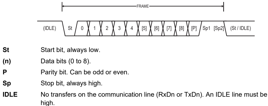
Figure 20-4. Frame Formats
