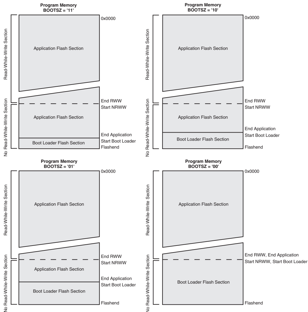
Figure 27-2. Memory Sections
