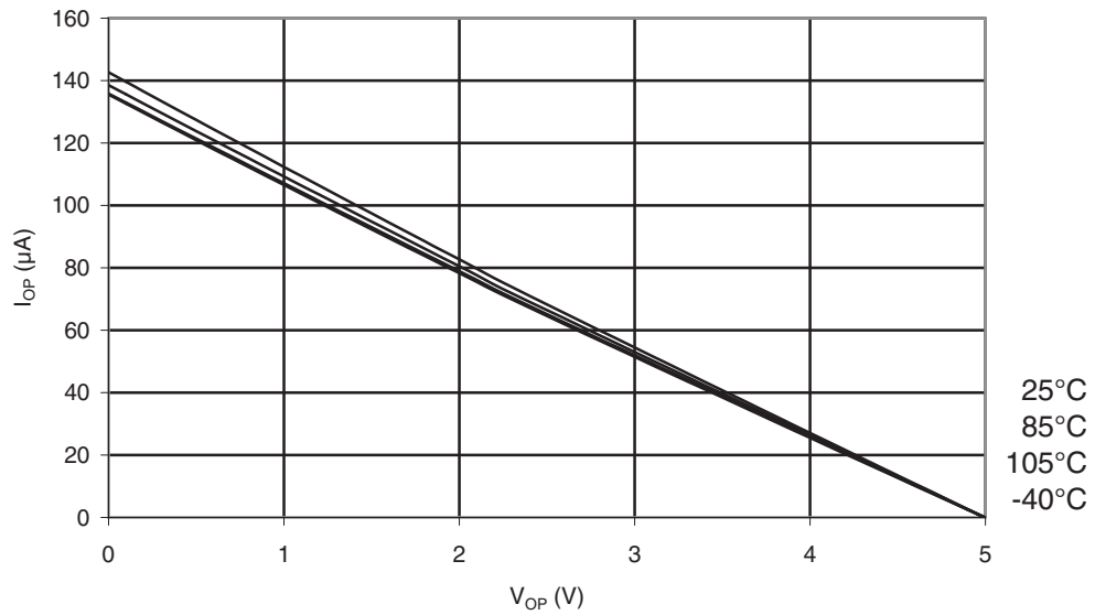
Figure 31-348. ATmega328P: I/O Pin Pull-up Resistor Current vs. Input Voltage ( V_{CC} = 5V )
