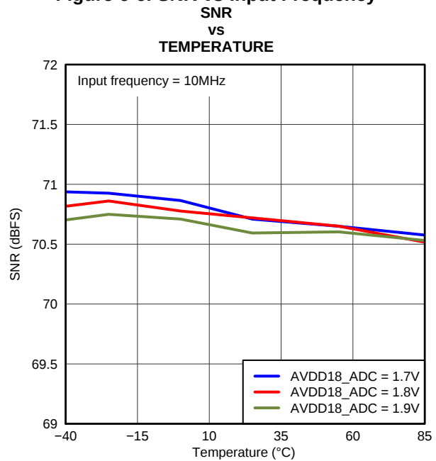
Figure 6-8. SNR Across Temperature and ADC Analog Supply
