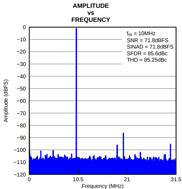
Figure 7-5. Spectrum With Decimation Filter ON SFDR
