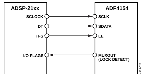
Figure 22. ADSP-21xx-to-ADF4154 Interface
