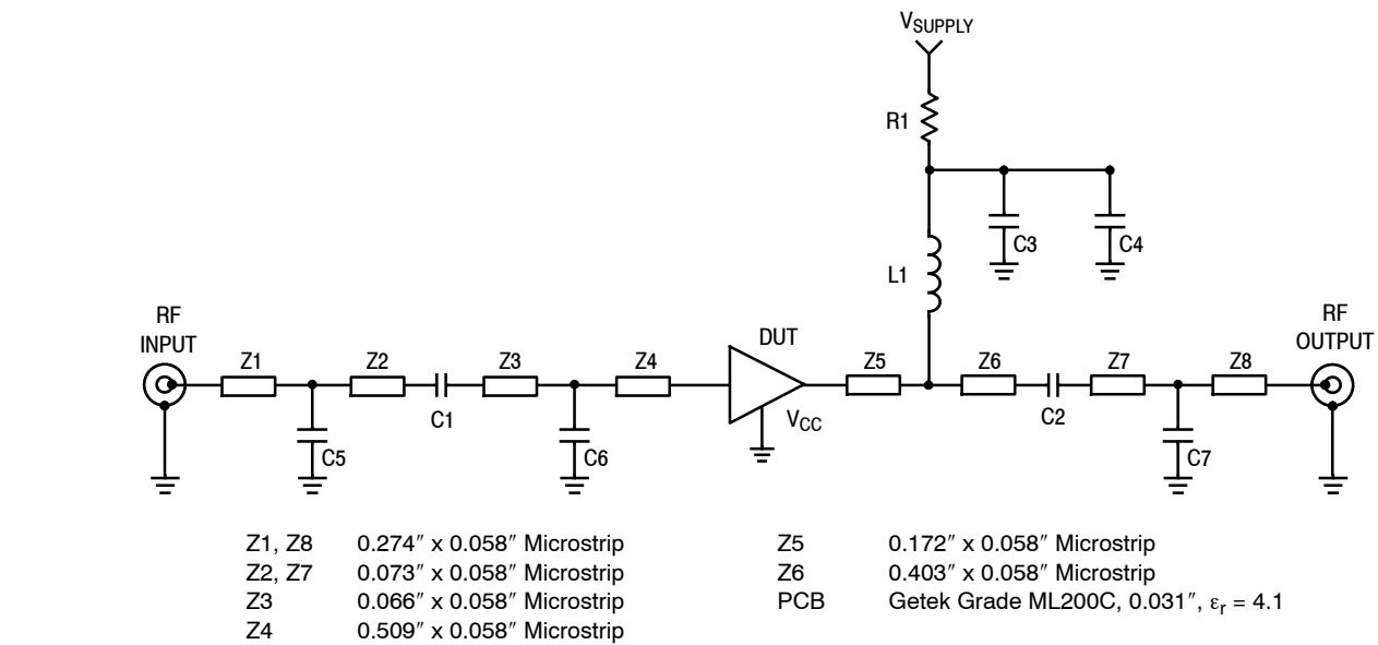
Figure 14. 50 Ohm Test Circuit Schematic
