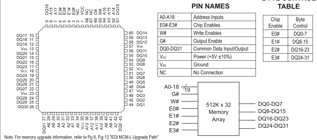
FIG. 1 PIN CONFIGURATIONS AND BLOCK DIAGRAM
