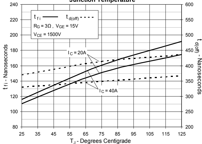
Fig. 20. Inductive Turn-off Switching Times vs. Junction Temperature
