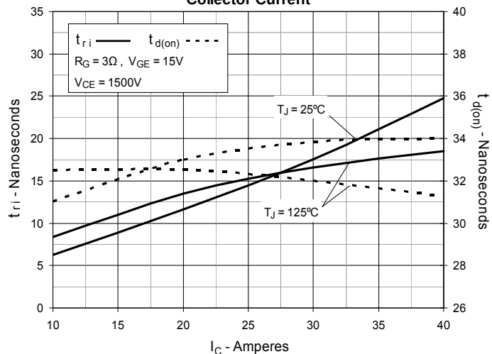
Fig. 22. Inductive Turn-on Switching Times vs. Collector Current
