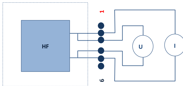
Fig. 10.1 Connection scheme for self-calibration procedure.
