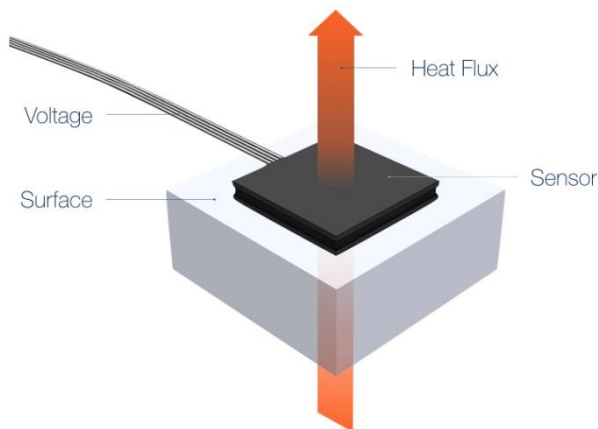
Fig. 7.1 Mounting onto solid surface
