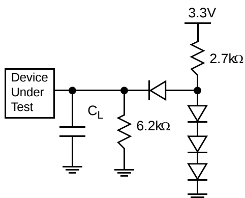
Figure 14. Test Setup
