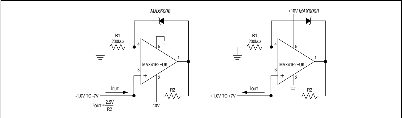
Figure 2. Precision 1μA to 1mA Current Sources
