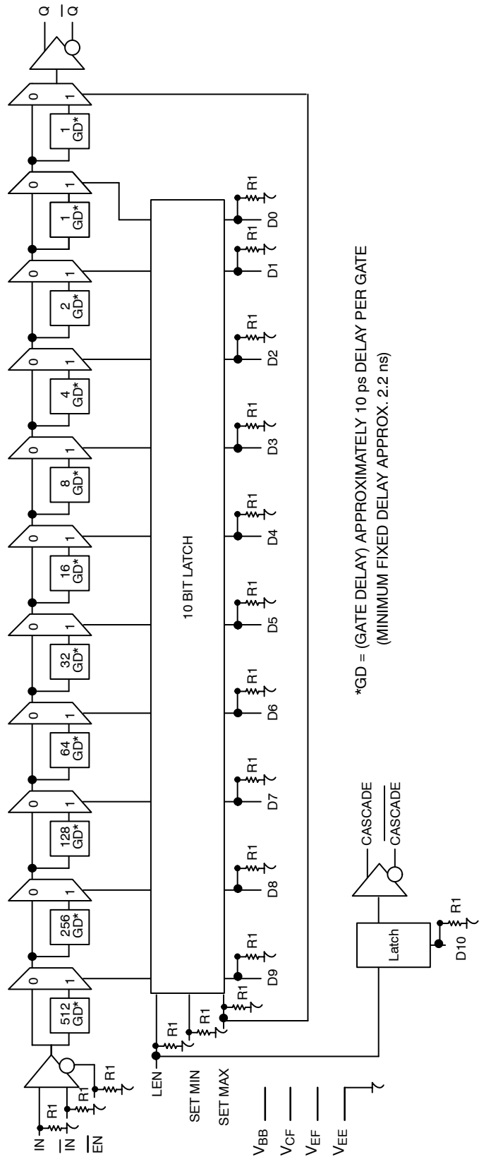
Figure 3. Logic Diagram
