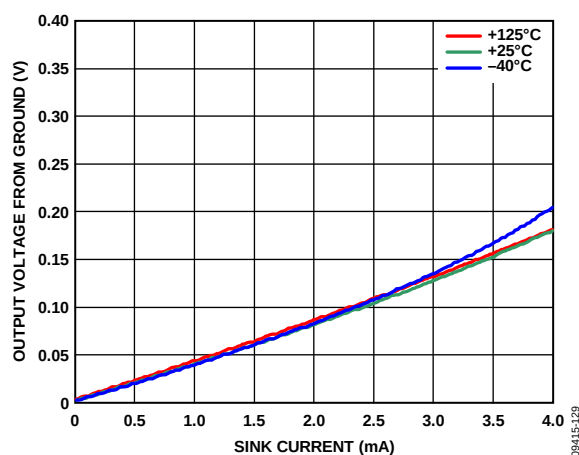
Figure 20. Output Voltage Range From Ground vs. Output Sink Current ( V_S = 5V )
