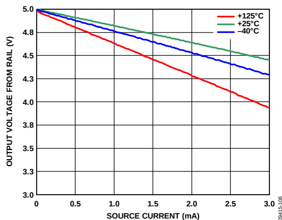
Figure 19. Output Voltage Range vs. Output Source Current ( V_S = 5V )
