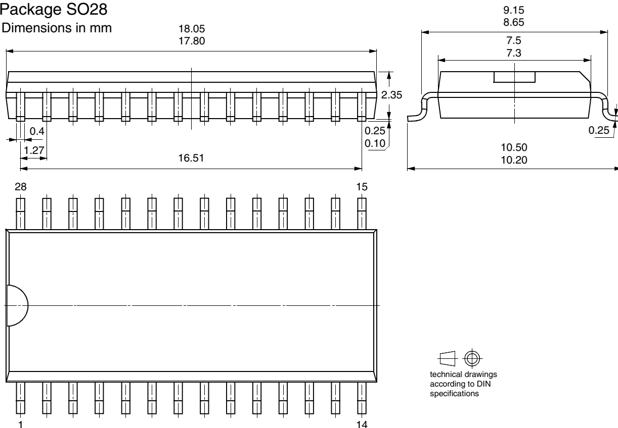
Figure 12-1. SO28
