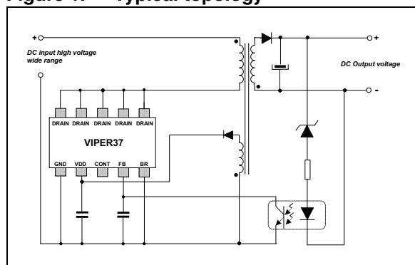
Figure 1. Typical topology
