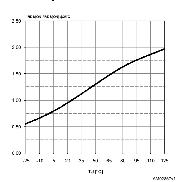
Figure 17. Power MOSFET ON resistance vs. T_J
