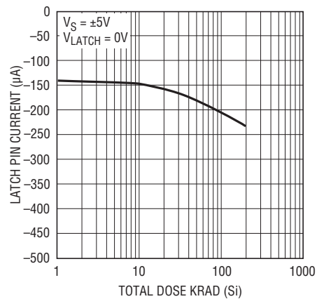
LATCH Pin Current
