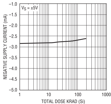
Negative Supply Current
