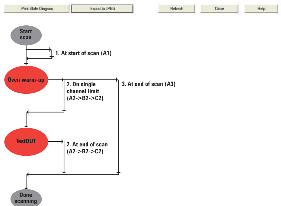
Figure 2. Oven control state diagram
