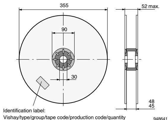
Figure 19. Reel Dimensions
