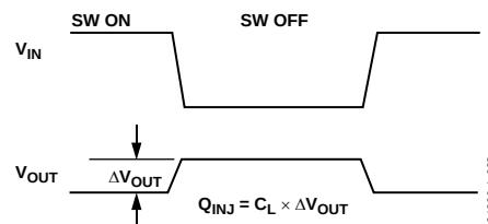
Figure 24. Charge Injection
