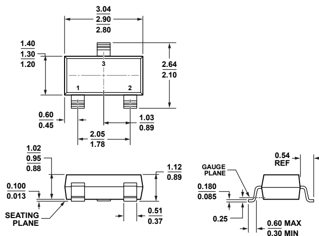
Figure 28. 3-Lead Small Outline Transistor Package [SOT-23-3] (RT-3)
