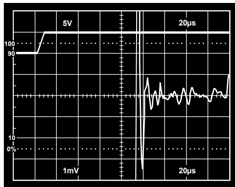
Figure 24. Turn-On Settling
