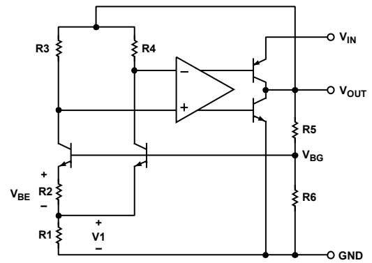
Figure 9. Simplified Schematic
