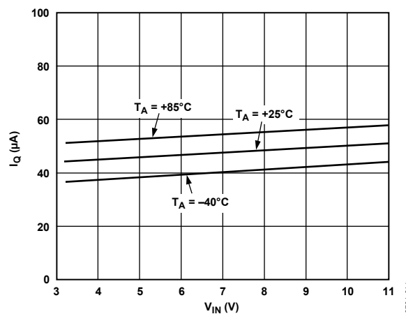
Figure 15. Typical Supply Current over Temperature
