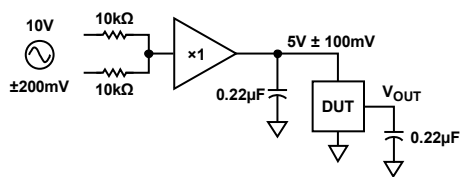
Figure 18. Ripple Rejection Test Circuit
