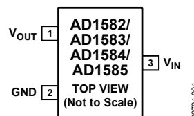
Figure 1. 3-Lead SOT-23-3 (RT Suffix)
