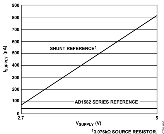
Figure 2. Supply Current ( \mu A) vs. Supply Voltage (V)
