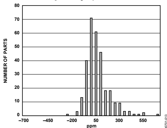
Figure 13. Output Voltage Hysteresis Distribution
