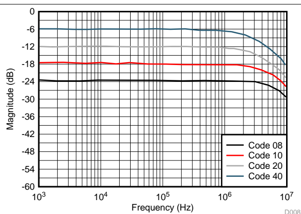
Figure 8. Frequency Response
