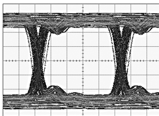
Figure 10. Equalized Signal (10m 24 AWG Twin-AX Cable, 3.2 Gbps, PRBS 7, 0x07 Setting)
