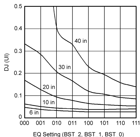
Figure 12. DJ vs. EQ Setting (3.2 Gbps)
