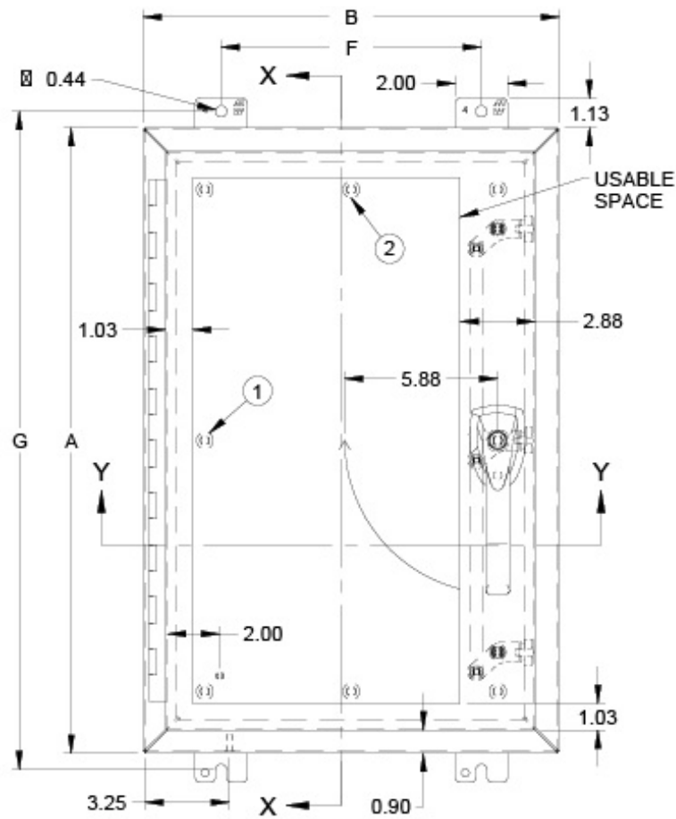
FRONT VIEW
