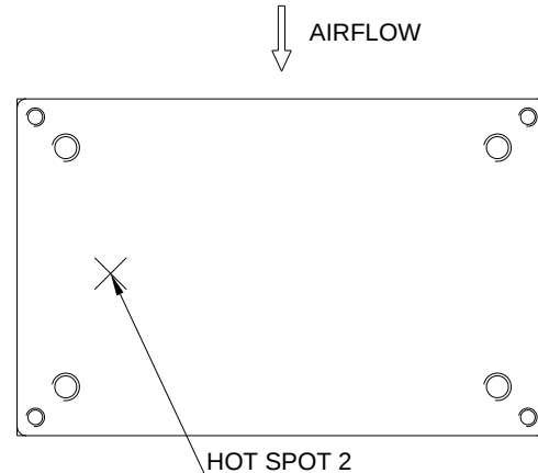
Figure 20: * Hot spot 2 temperature measured point. The allowed maximum hot spot 2 temperature is defined at 112 °C
