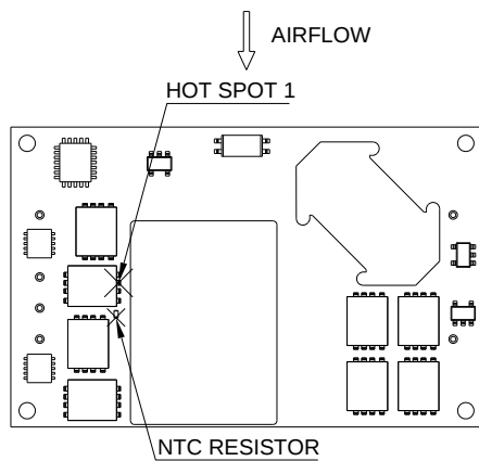
Figure 18: * Hot spot 1& NTC resistor temperature measured points. The allowed maximum hot spot 1 temperature is defined at 121 °C
