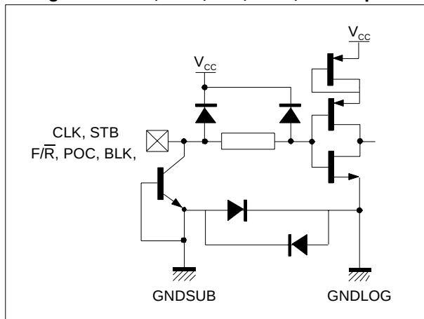
Figure 7: CLK, STB, \overline{F/R} , POC, BLK inputs
