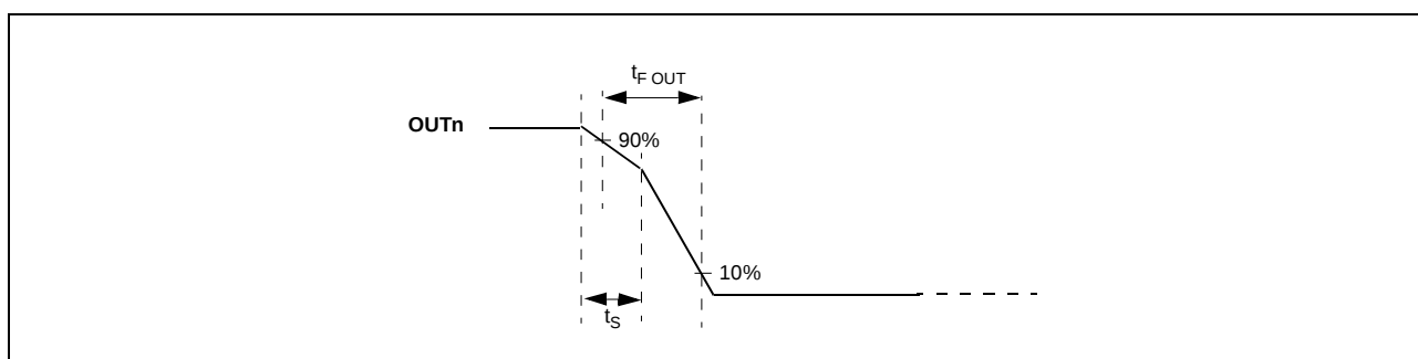
Figure 6: Zoom for OUTn showing t_S and t_{F\text{ OUT}}
