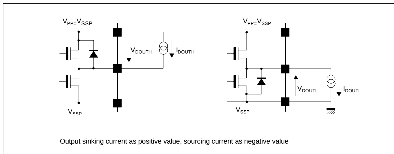
Figure 5: Test configuration
