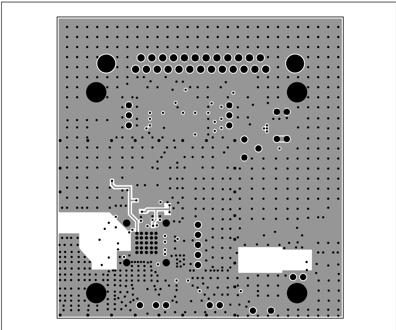
Figure 4. MAX3541/MAX3542 EV Kits PCB Layout—Inner Layer 2
