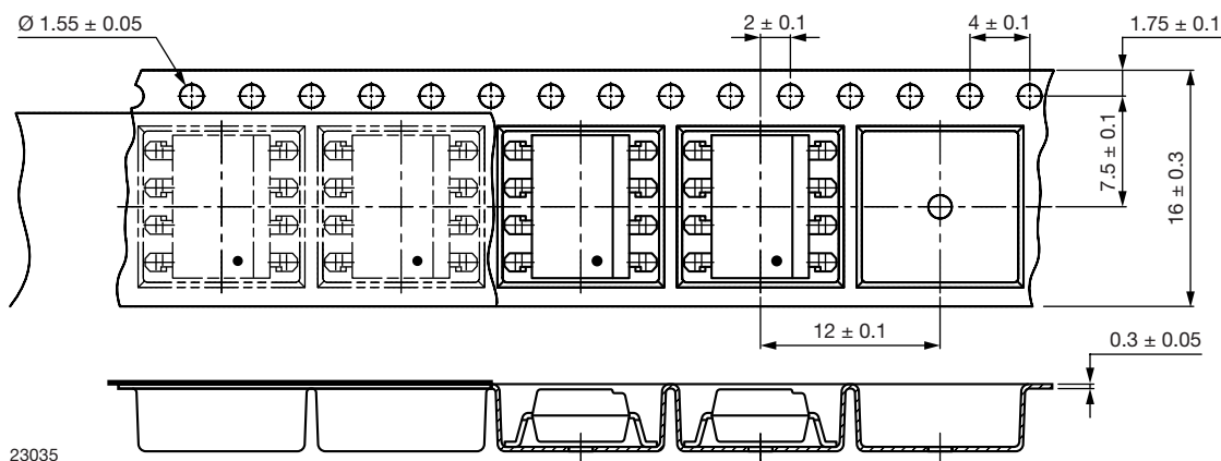
Fig. 21 - Tape and Reel Packaging (1000 pieces on reel)
