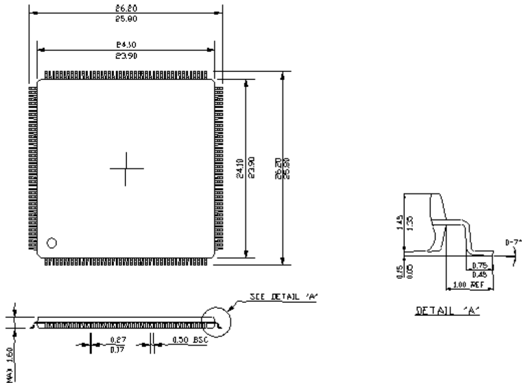
Figure 4. Physical Dimensions
