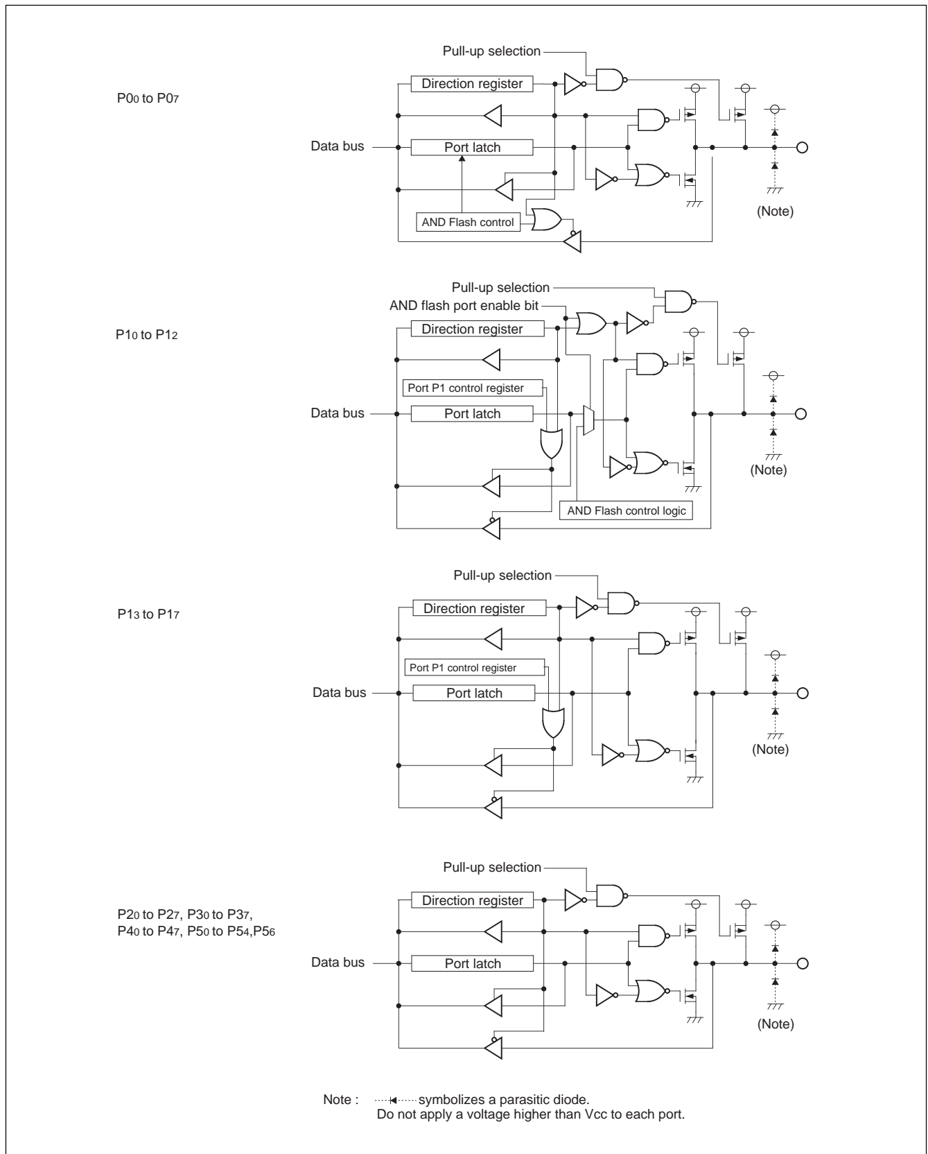
Figure 1.132. Programmable I/O ports (1)
