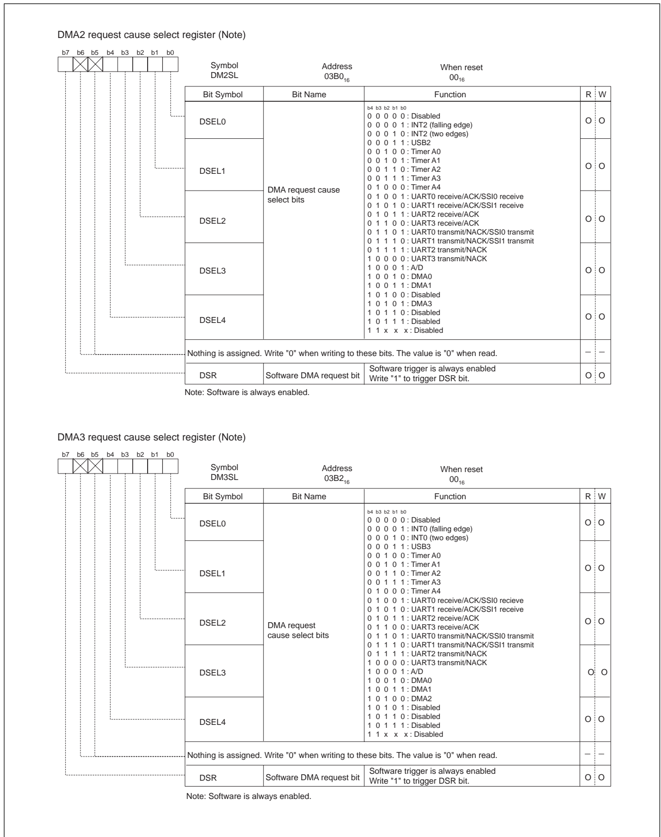
Figure 1.72. DMAC register (2)
