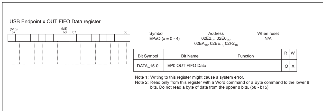
Figure 1.66. USB Endpoint x OUT FIFO Data register (EPxO)
