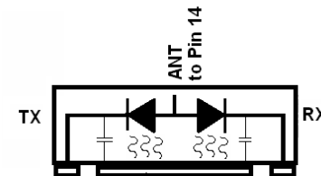
Thermal Ground for Diodes Electrical ground for internal matching components
