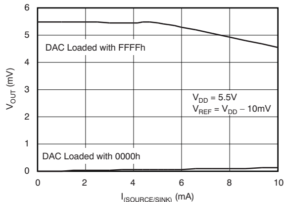
Figure 7. Source and Sink Current Capability
