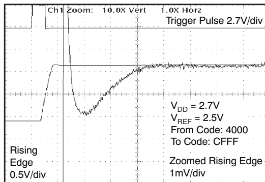
Figure 38. Half-Scale Settling Time: Rising Edge
