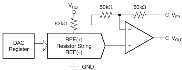
Figure 46. DAC8550 Architecture
