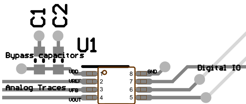
Figure 59. Layout Diagram
