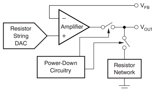
Figure 48. Output Stage During Power-Down
