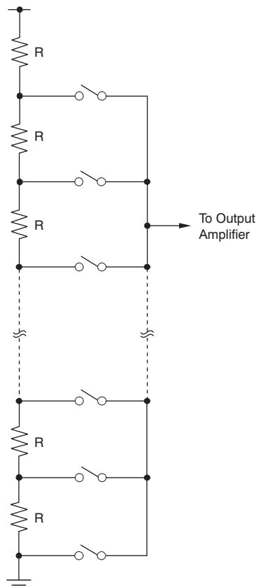
Figure 47. Resistor String
