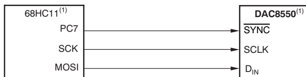
Figure 58. DAC8550 to 68HC11 Interface
