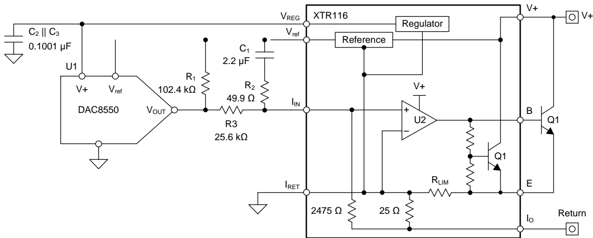
Figure 52. Loop-Powered Transmitter
