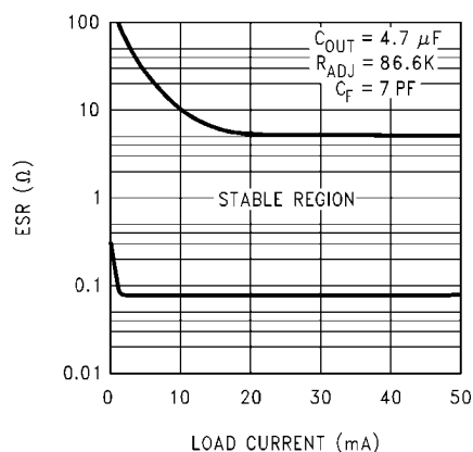
4.7 \mu F ESR Curves
