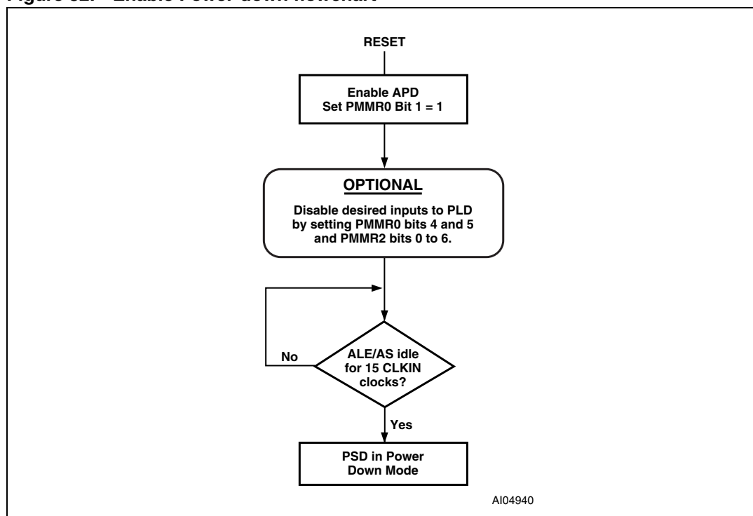
Figure 32. Enable Power-down flowchart
