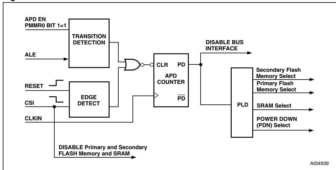
Figure 31. APD unit
