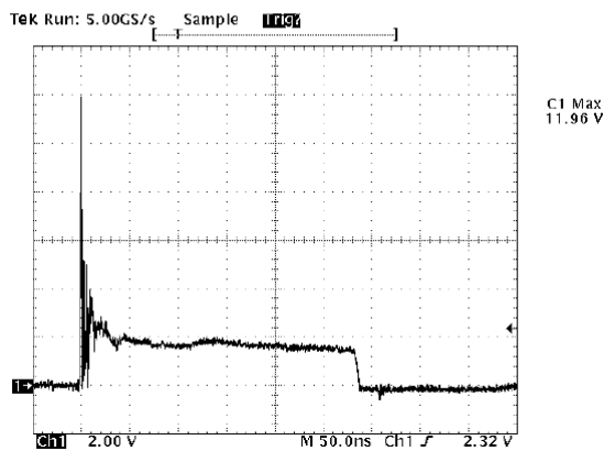
Fig5 - ESD Clamping (+8KV Contac per IEC61000-4-2)
