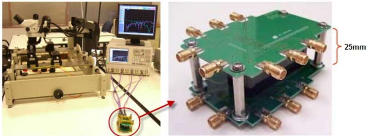
Figure 98 Measurement setup
