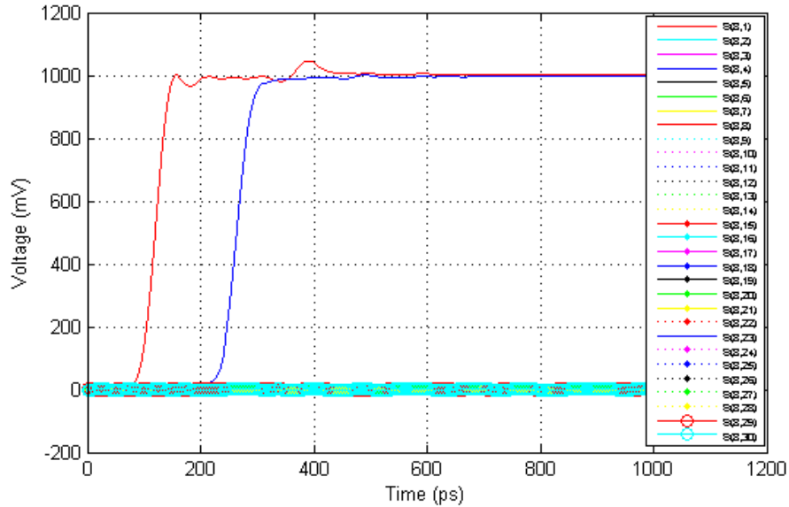
Figure 51 TDR and TDT waveforms @30ps rise time (20% to 80%) and 10.5GHz BW for pair 8 of IT3-25mm
