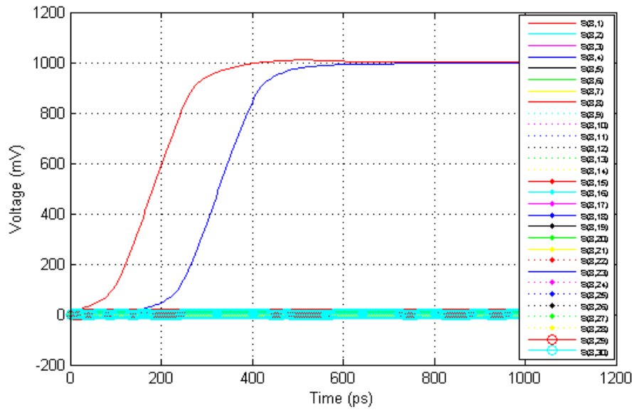
Figure 53 TDR and TDT waveforms @120ps rise time (20% to 80%) and 2.625GHz BW for pair 8 of IT3-25mm
