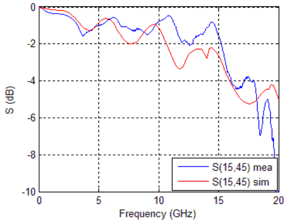
Figure 112 Measurement vs. simulation correlation of IL and RL for center port (for IT3-25mm) as shown in Figure 111
