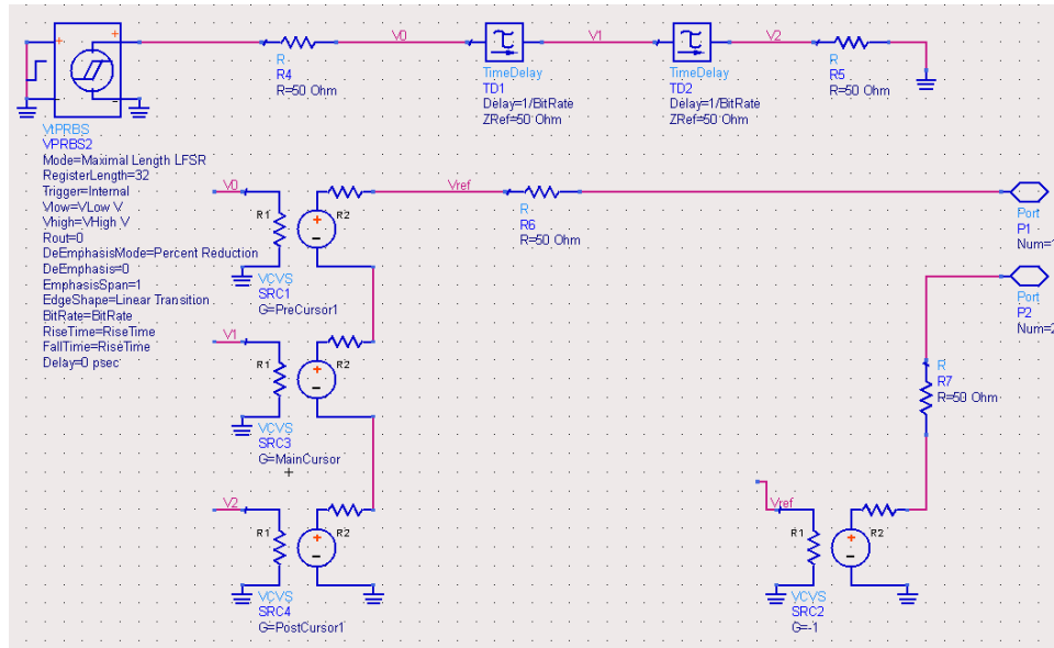
Figure 118 3-tap transmitter equalization setup
