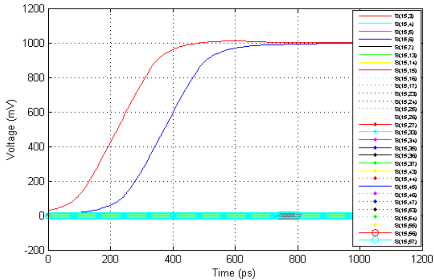
Figure 95 TDR and TDT waveforms @180ps rise time (20% to 80%) and 1.75GHz BW for port 15 of IT3-25mm
