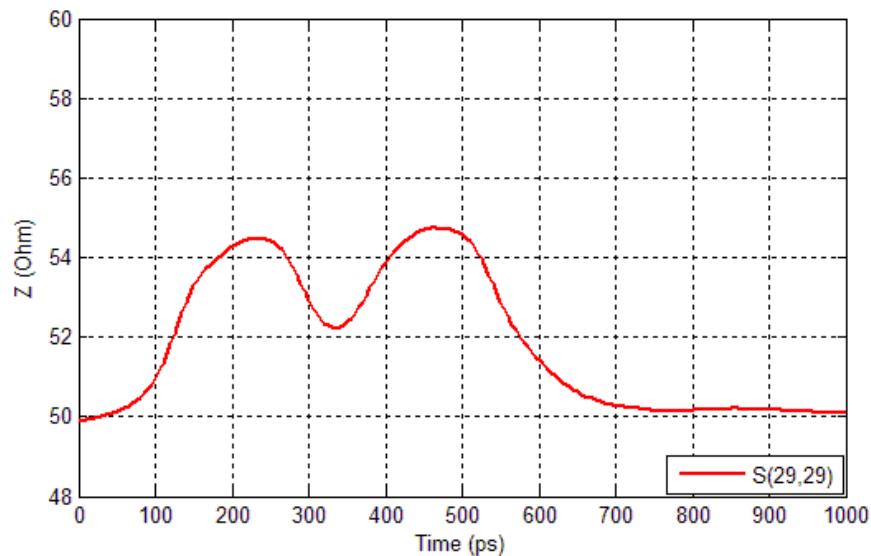
Figure 87 Impedance profile for top edge port 29 of IT3-25mm (connector only) @120ps rise time (20% to 80%) and 2.625GHz BW
