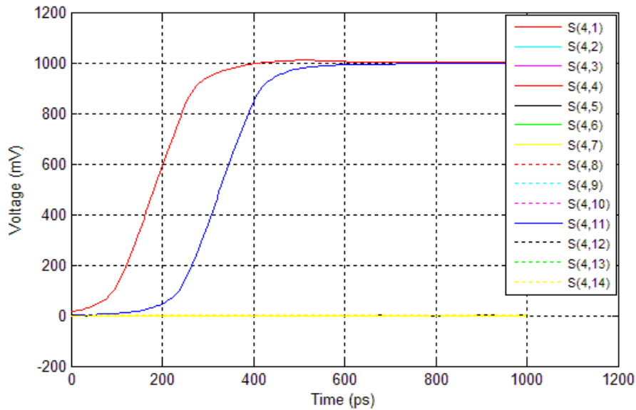
Figure 59 TDR and TDT waveforms @120ps rise time (20% to 80%) and 2.625GHz BW for pair 4 of IT3-25mm for 50% pin density configuration
