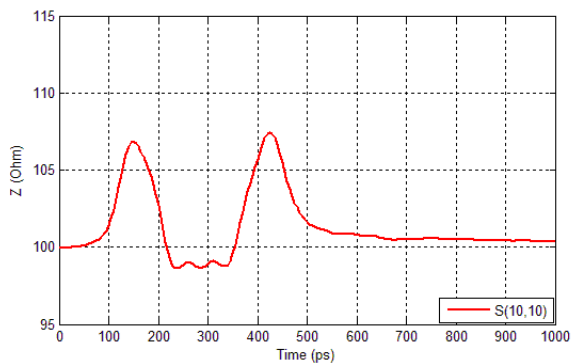
Figure 44 Impedance profile for right edge pair 10 of IT3-25mm (connector only) @60ps rise time (20% to 80%) and 5.25GHz BW, and @30ps rise time (20% to 80%) and 10.5GHz BW
