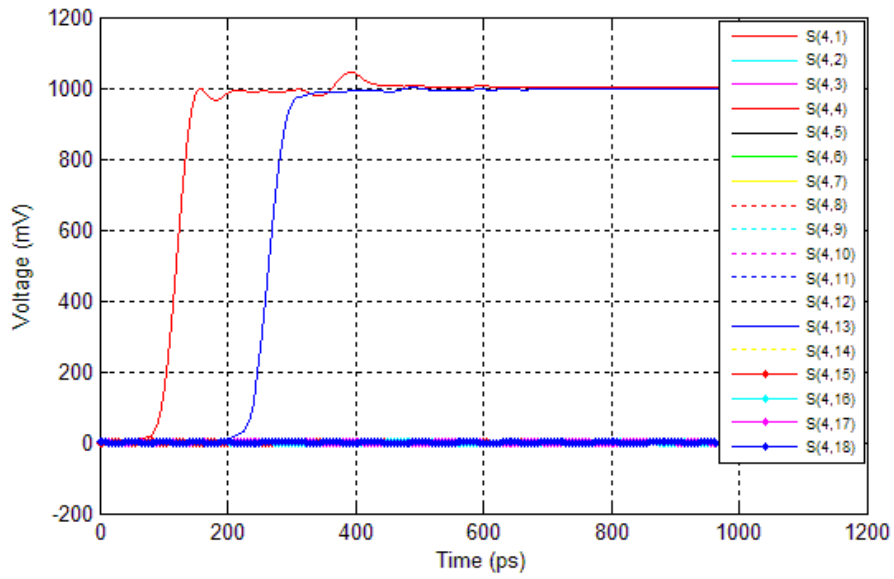
Figure 54 TDR and TDT waveforms @30ps rise time (20% to 80%) and 10.5GHz BW for pair 4 of IT3-25mm for 60% pin density configuration
