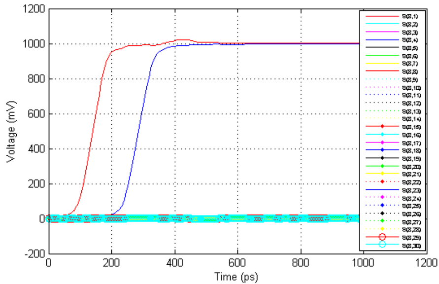
Figure 52 TDR and TDT waveforms @60ps rise time (20% to 80%) and 5.25GHz BW for pair 8 of IT3-25mm
