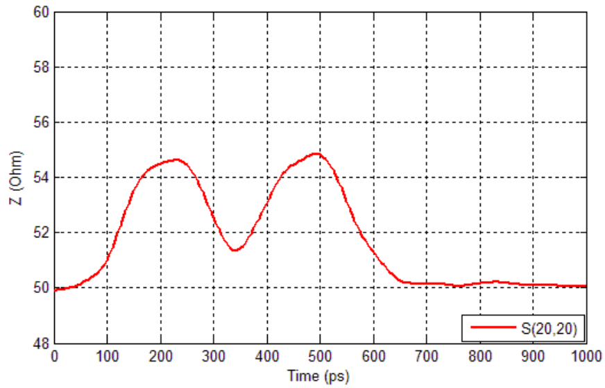
Figure 86 Impedance profile for right edge port 20 of IT3-25mm (connector only) @120ps rise time (20% to 80%) and 2.625GHz BW
