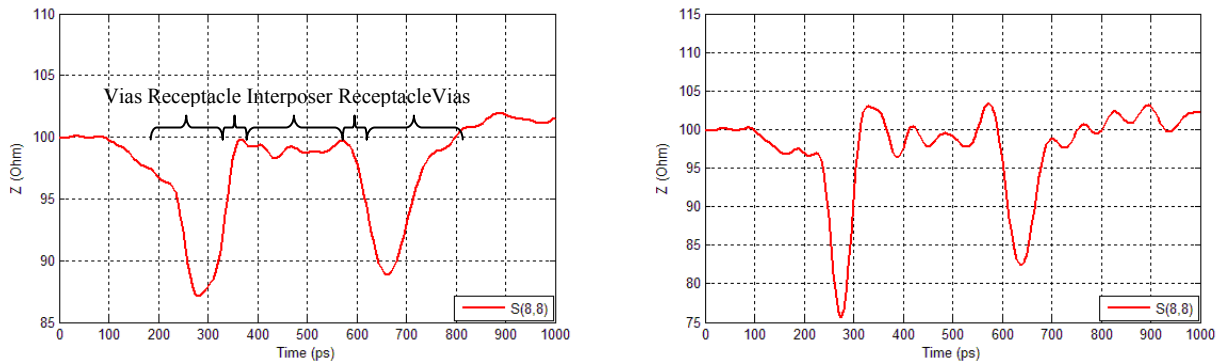
Figure 47 Impedance profile for center pair 8 of IT3-25mm (vias+connector+vias) with routing on layer 16 @60ps rise time (20% to 80%) and 5.25GHz BW, and @30ps rise time (20% to 80%) and 10.5GHz BW
