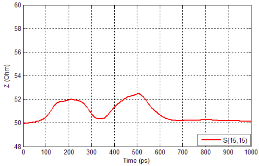
Figure 85 Impedance profile for center port 15 of IT3-25mm (connector only) @120ps rise time (20% to 80%) and 2.625GHz BW
