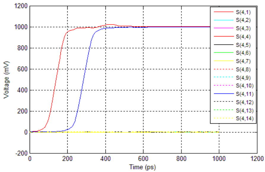
Figure 58 TDR and TDT waveforms @60ps rise time (20% to 80%) and 5.25GHz BW for pair 4 of IT3-25mm for 50% pin density configuration
