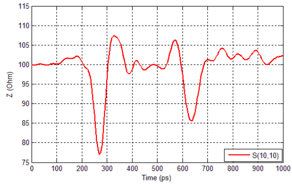
Figure 48 Impedance profile for right edge pair 10 of IT3-25mm (vias+connector+vias) with routing on layer 16 @60ps rise time (20% to 80%) and 5.25GHz z BW, and @30ps rise time (20% to 80%) and 10.5GHz z BW
