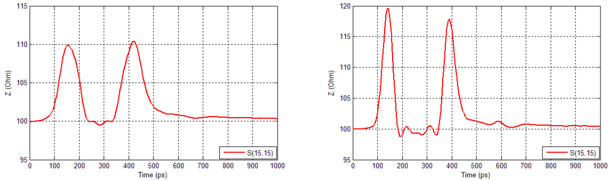
Figure 46 Impedance profile for top corner pair 15 of IT3-25mm (connector only) @60ps rise time (20% to 80%) and 5.25GHz BW, and @30ps rise time (20% to 80%) and 10.5GHz BW
