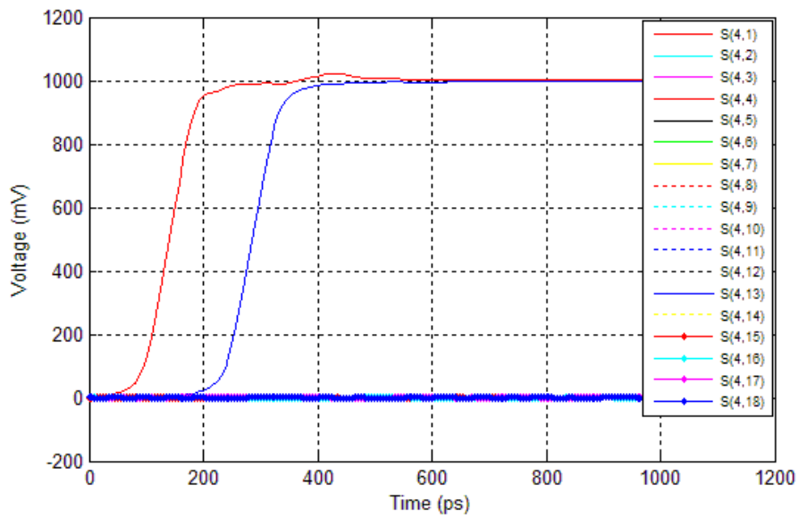
Figure 55 TDR and TDT waveforms @60ps rise time (20% to 80%) and 5.25GHz BW for pair 4 of IT3-25mm for 60% pin density configuration
