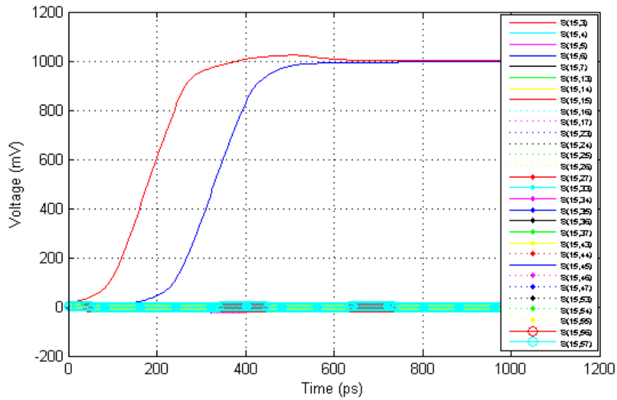
Figure 93 TDR and TDT waveforms @120ps rise time (20% to 80%) and 2.625GHz BW for port 15 of IT3-25mm
