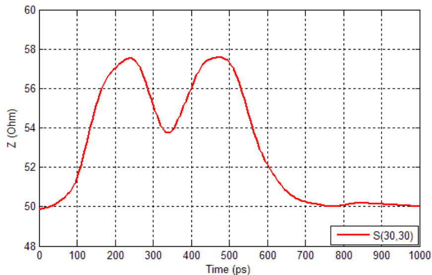
Figure 88 Impedance profile for top corner port 30 of IT3-25mm (connector only) @120ps rise time (20% to 80%) and 2.625GHz BW
