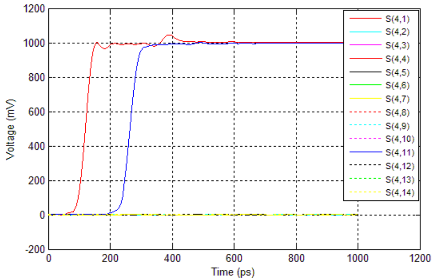
Figure 57 TDR and TDT waveforms @30ps rise time (20% to 80%) and 10.5GHz BW for pair 4 of IT3-25mm for 50% pin density configuration
