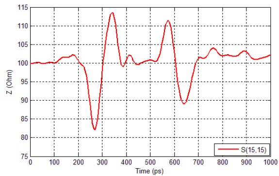
Figure 50 Impedance profile for top corner pair 15 of IT3-25mm (vias+connector+vias) with routing on layer 19 @60ps rise time (20% to 80%) and 5.25GHz z BW, and @30ps rise time (20% to 80%) and 10.5GHz z BW
