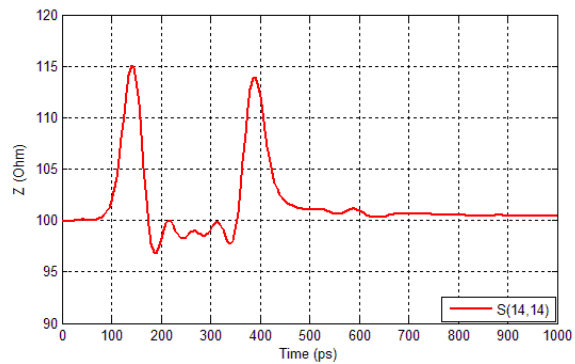
Figure 45 Impedance profile for top edge pair 14 of IT3-25mm (connector only) @60ps rise time (20% to 80%) and 5.25GHz BW, and @30ps rise time (20% to 80%) and 10.5GHz BW
