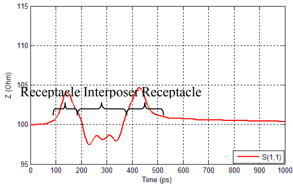
Figure 43 Impedance profile for center pair 8 of IT3-25mm (connector only) @60ps rise time (20% to 80%) and 5.25GHz BW, and @30ps rise time (20% to 80%) and 10.5GHz BW
