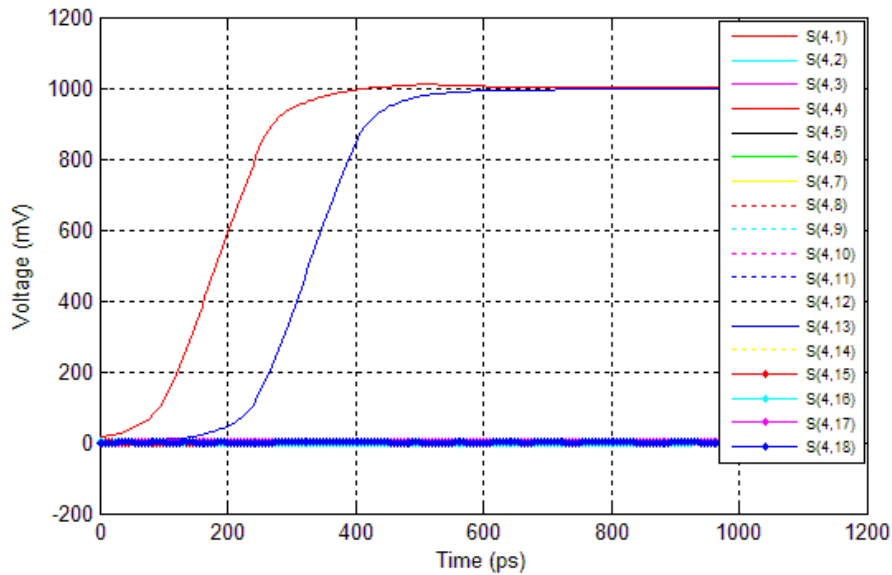
Figure 56 TDR and TDT waveforms @120ps rise time (20% to 80%) and 2.625GHz for pair 4 of IT3-25mm for 60% pin density configuration
