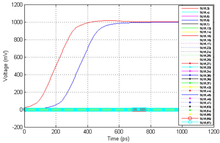
Figure 94 TDR and TDT waveforms @150ps rise time (20% to 80%) and 2.1GHz BW for port 15 of IT3-25mm
