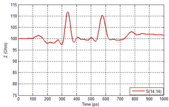
Figure 49 Impedance profile for top edge pair 14 of IT3-25mm (vias+connector+vias) with routing on layer 28 @60ps rise time (20% to 80%) and 5.25GHz z BW, and @30ps rise time (20% to 80%) and 10.5GHz z BW
