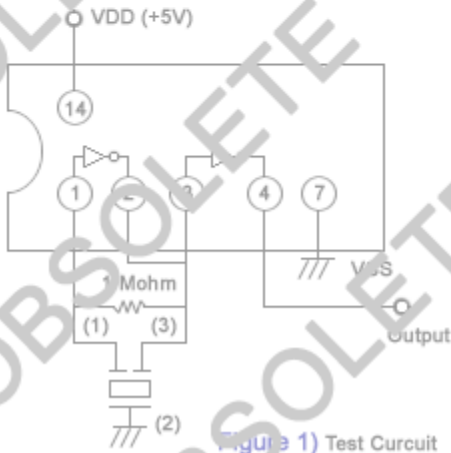
Figure 1) Test Curcuit
