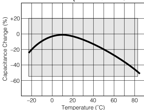
Char. E/Y5U ( Temp.Range:-25 to 85 °C max.Cap.Change:+20, -55 % )
