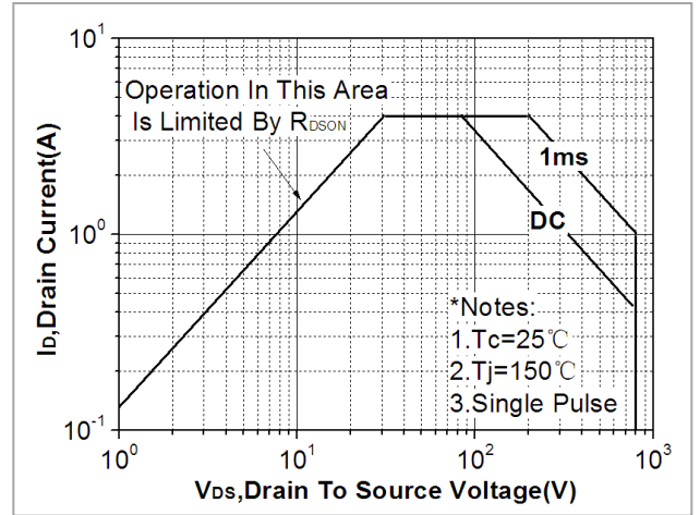
Fig. 8. Maximum safe operating area(TO-251N)
