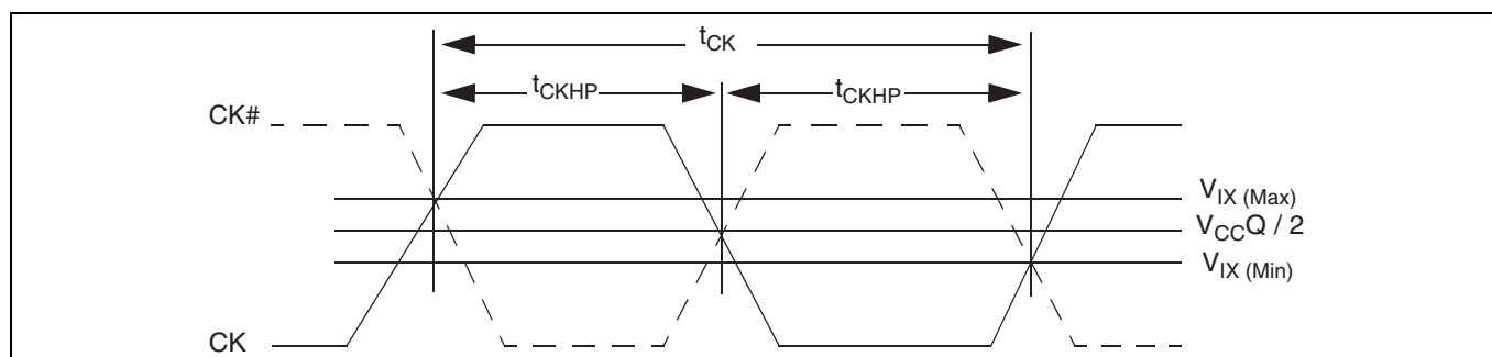
Figure 28 Clock characteristics
