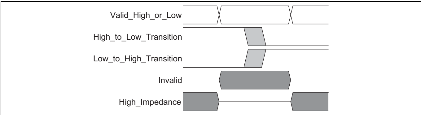
Figure 25 Key to switching waveforms
