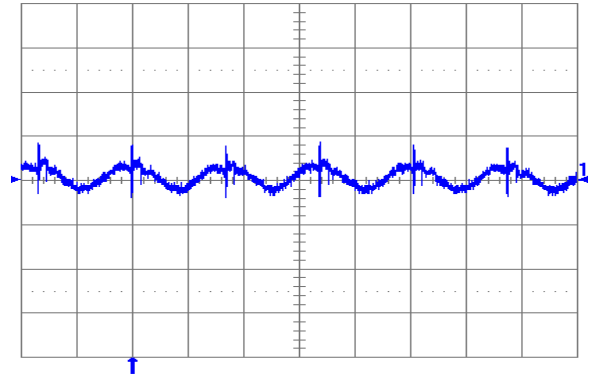
Fig. 1.0V.6: Output voltage ripple (20 mV/div.) at full rated load current into a resistive load with external capacitance 100\text{ }\mu\text{F} ceramic + 1\text{ }\mu\text{F} ceramic, and V_{in} = 12 V for V_{out} = 1.0 V. Time scale: 2\text{ }\mu\text{s/div.}
