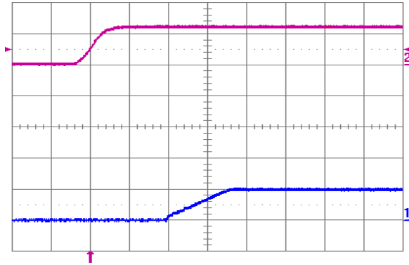
Fig. 1.0V.5: Turn-on transient for V_{out} = 1.0 V with application of V_{in} at full rated load current (resistive) and 100\text{ }\mu\text{F} external capacitance at V_{in} = 12 V. Top trace: V_{in} (10 V/div.); Bottom trace: output voltage (1 V/div.); Time scale: 2 ms/div.
