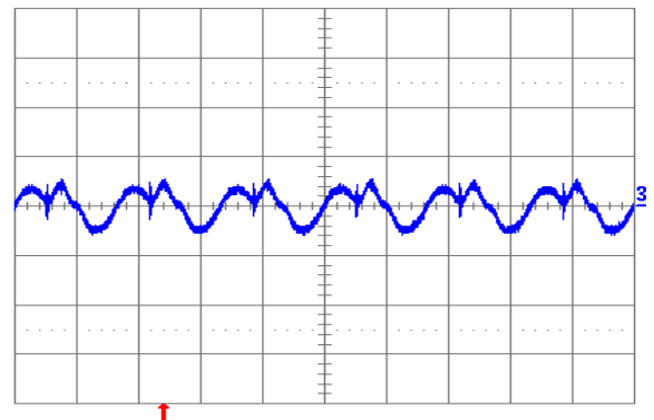
Fig. 1.5V.6: Output voltage ripple (20 mV/div.) at full rated load current into a resistive load with external capacitance 100 \mu F ceramic + 1 \mu F ceramic, and V_{in} = 12 V for V_{out} = 1.5 V. Time scale: 2 \mu s/div.
