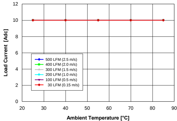
Fig. 2.0V.1: Available load current vs. ambient temperature and airflow rates for V_{out} = 2.0 V converter mounted vertically with V_{in} = 12 V, and maximum MOSFET temperature \leq 110 °C.
