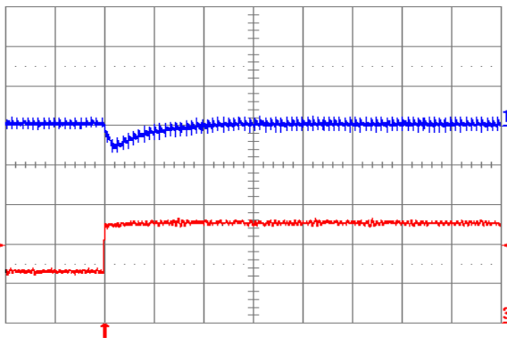
Fig. 1.8V.7: Output voltage response for V_{out} = 1.8 V to positive load current step change from 5 A to 10 A with slew rate of 5 \text{ A}/\mu\text{s} at V_{in} = 12 V. Top trace: output voltage (100 mV/div.); Bottom trace: load current (5 A/div.). C_o = 100 \mu\text{F} ceramic. Time scale: 20 \mu\text{s}/\text{div} .
