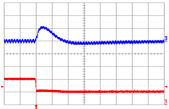
Fig. 1.5V.8: Output voltage response for V_{out} = 1.5 V to negative load current step change from 10 A to 5 A with slew rate of -5 A/ \mu s at V_{in} = 12 V. Top trace: output voltage (100 mV/div.); Bottom trace: load current (2 A/div.). C_o = 100 \mu F ceramic. Time scale: 20 \mu s/div.
