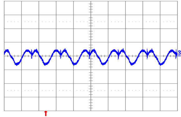
Fig. 1.8V.6: Output voltage ripple (20 mV/div.) at full rated load current into a resistive load with external capacitance 100 \mu\text{F} ceramic + 1 \mu\text{F} ceramic, and V_{in} = 12 V for V_{out} = 1.8 V. Time scale: 2 \mu\text{s}/\text{div} .
