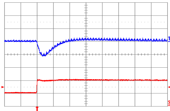
Fig. 0.7525V.7: Output voltage response for V_{out} = 0.7525 V to positive load current step change from 5 A to 10 A with slew rate of 5 A/ \mu s at V_{in} = 12 V. Top trace: output voltage (100 mV/div.); Bottom trace: load current (5 A/div.). C_o = 100 \mu F ceramic. Time scale: 20 \mu s/div.
