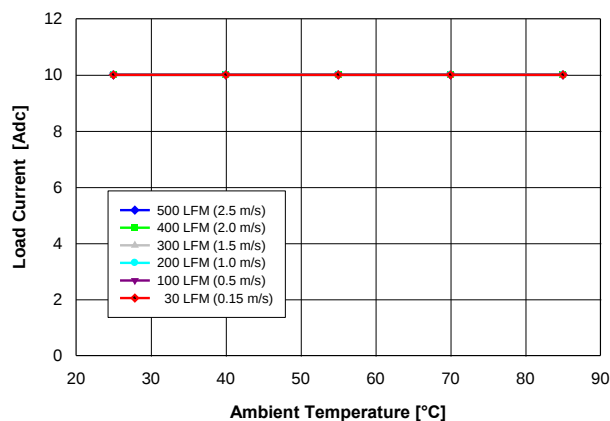
Fig. 0.7525V.1: Available load current vs. ambient temperature and airflow rates for V_{out} = 0.7525 V converter mounted vertically with V_{in} = 12 V, and maximum MOSFET temperature \leq 110\text{ }^{\circ}\text{C} .
