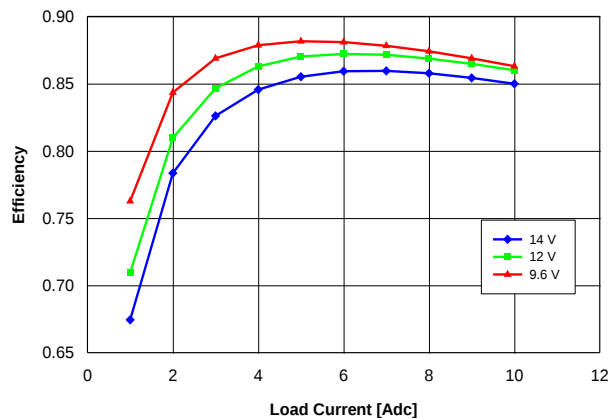
Fig. 1.0V.3: Efficiency vs. load current and input voltage for V_{out} = 1.0 V converter mounted vertically with air flowing at a rate of 200 LFM (1 m/s) and T_a = 25 ^{\circ} C.
