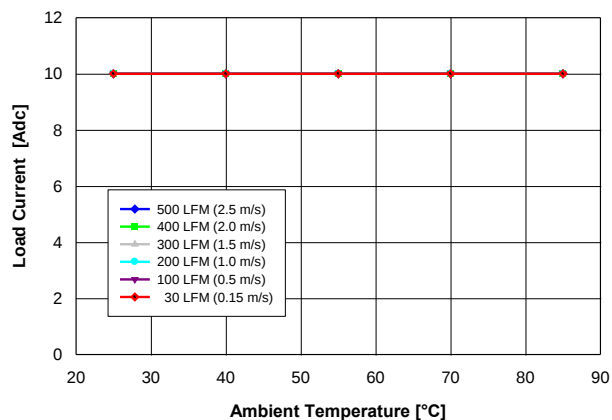
Fig. 2.5V.1: Available load current vs. ambient temperature and airflow rates for V_{out} = 2.5\text{ V} converter mounted vertically with V_{in} = 12\text{ V} , and maximum MOSFET temperature \leq 110\text{ }^{\circ}\text{C} .
