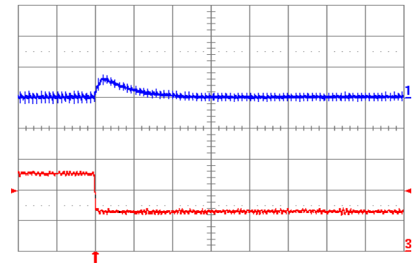
Fig. 1.8V.8: Output voltage response for V_{out} = 1.8 V to negative load current step change from 10 A to 5 A with slew rate of -5 \text{ A}/\mu\text{s} at V_{in} = 12 V. Top trace: output voltage (100 mV/div.); Bottom trace: load current (5 A/div.). C_o = 100 \mu\text{F} ceramic. Time scale: 20 \mu\text{s}/\text{div} .
