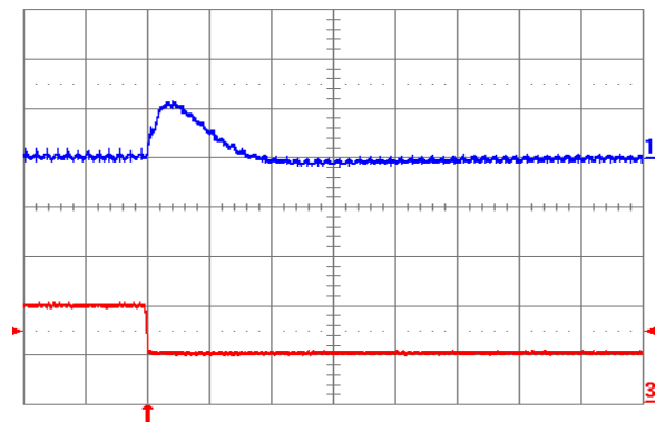
Fig. 1.0V.8: Output voltage response for V_{out} = 1.0 V to negative load current step change from 10 A to 5 A with slew rate of -5\text{ A}/\mu\text{s} at V_{in} = 12 V. Top trace: output voltage (100 mV/div.); Bottom trace: load current (5 A/div.). C_o = 100\text{ }\mu\text{F} ceramic. Time scale: 20\text{ }\mu\text{s/div.}
