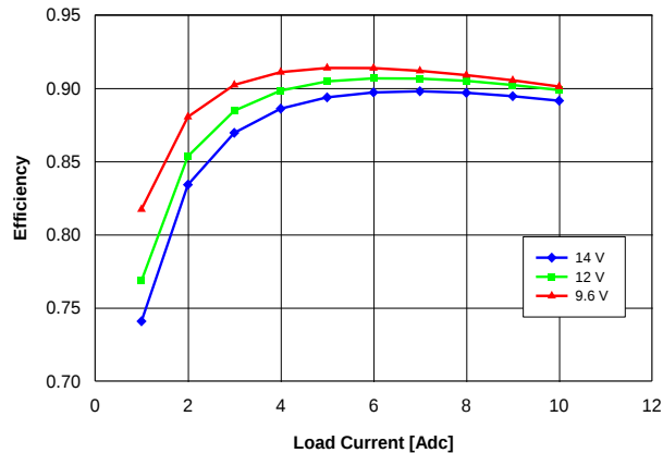
Fig. 1.5V.3: Efficiency vs. load current and input voltage for V_{out} = 1.5 V converter mounted vertically with air flowing at a rate of 200 LFM (1 m/s) and T_a = 25 °C.
