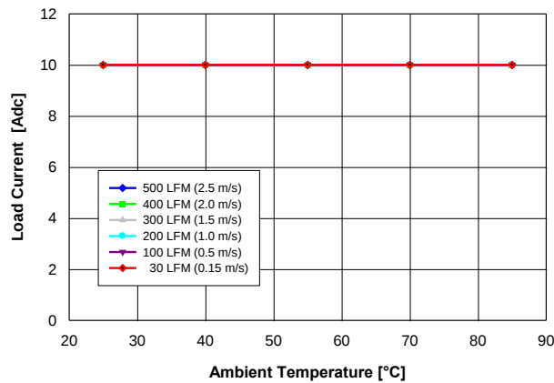
Fig. 1.0V.1: Available load current vs. ambient temperature and airflow rates for V_{out} = 1.0 V converter mounted vertically with V_{in} = 12 V, and maximum MOSFET temperature \leq 110 ^{\circ} C.
