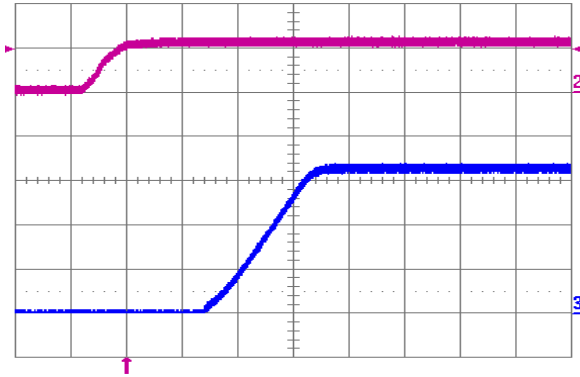
Fig. 3.3V.5: Turn-on transient for V_{out} = 3.3\text{ V} with application of V_{in} at full rated load current (resistive) and 100\text{ }\mu\text{F} external capacitance at V_{in} = 12\text{ V} . Top trace: V_{in} ( 10\text{ V/div.} ); Bottom trace: output voltage ( 1\text{ V/div.} ); Time scale: 2\text{ ms/div.}
