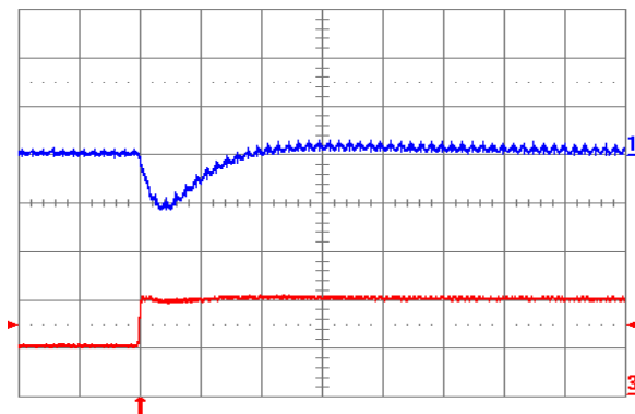
Fig. 1.0V.7: Output voltage response for V_{out} = 1.0 V to positive load current step change from 5 A to 10 A with slew rate of 5\text{ A}/\mu\text{s} at V_{in} = 12 V. Top trace: output voltage (100 mV/div.); Bottom trace: load current (5 A/div.). C_o = 100\text{ }\mu\text{F} ceramic. Time scale: 20\text{ }\mu\text{s/div.}
