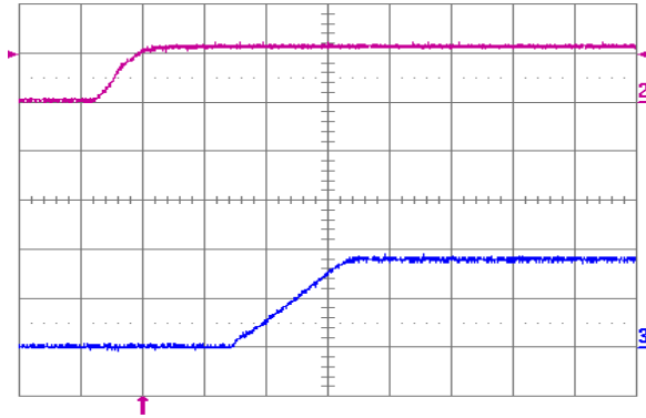
Fig. 1.8V.5: Turn-on transient for V_{out} = 1.8 V with application of V_{in} at full rated load current (resistive) and 100 \mu\text{F} external capacitance at V_{in} = 12 V. Top trace: V_{in} (10 V/div.); Bottom trace: output voltage (1 V/div.); Time scale: 2 ms/div.
