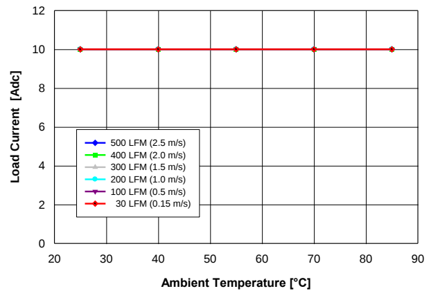
Fig. 1.0V.2: Available load current vs. ambient temperature and airflow rates for V_{out} = 1.0 V converter mounted horizontally with V_{in} = 12 V, and maximum MOSFET temperature \leq 110 ^{\circ} C.
