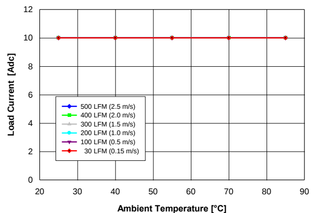
Fig. 0.7525V.2: Available load current vs. ambient temperature and airflow rates for V_{out} = 0.7525 V converter mounted horizontally with V_{in} = 12 V, and maximum MOSFET temperature \leq 110\text{ }^{\circ}\text{C} .
