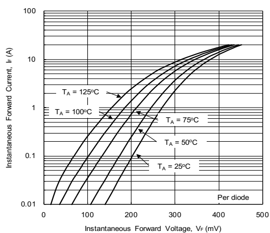
Fig. 1 - Forward Characteristics
