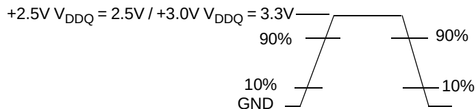
Figure 20-1. Input Waveform for CYNSE70032
