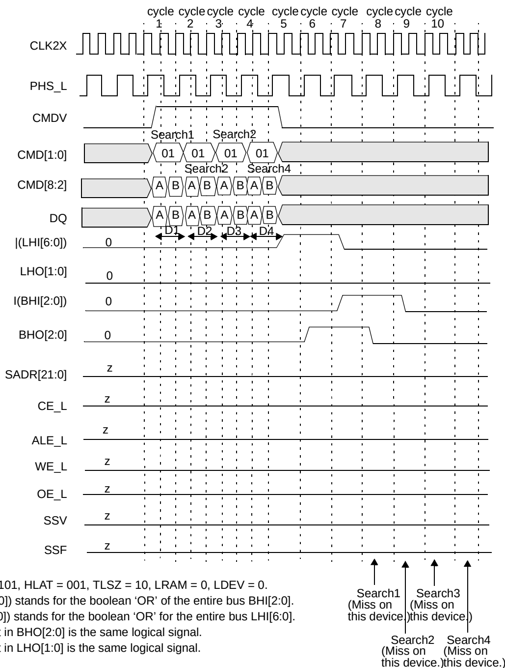
Figure 13-42. Timing Diagram for Devices Below the Winning Device in Block Number 3 Except Device Number 30 (the Last Device)
