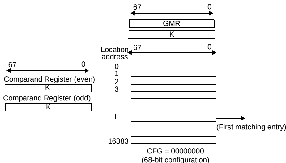
Figure 13-3. ×68 Table with One Device
