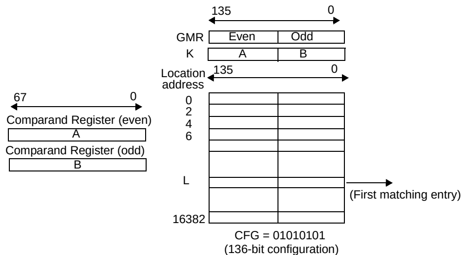
Figure 13-25. ×136 Table with One Device
