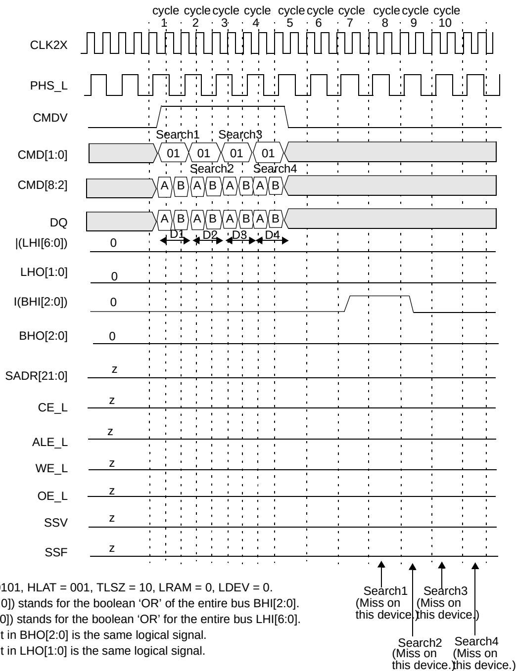
Figure 13-40. Timing Diagram for Devices Above the Winning Device in Block Number 3
