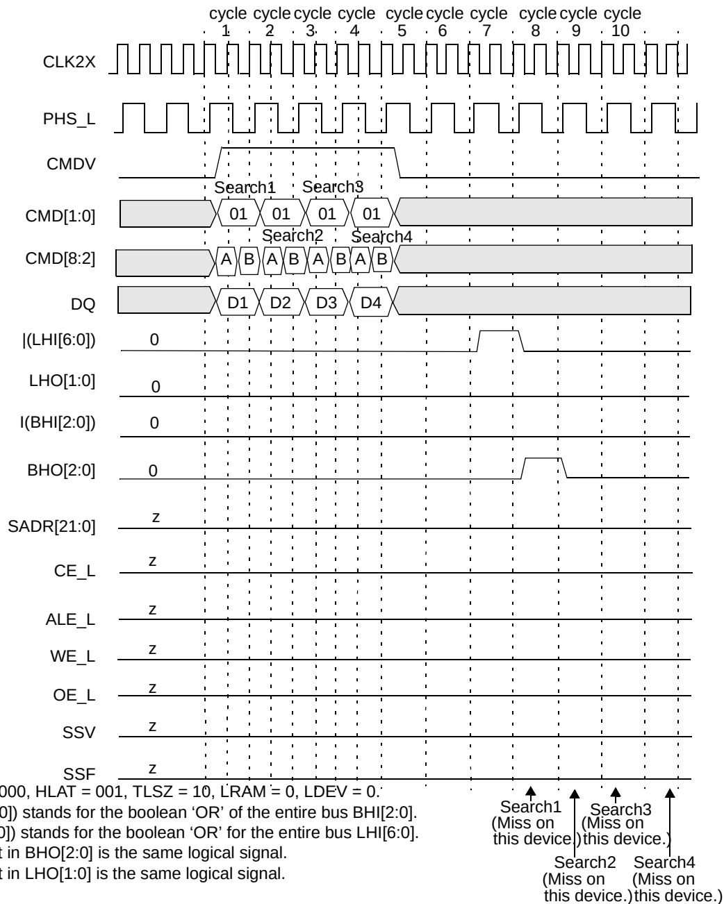
Figure 13-14. Timing Diagram for Devices Below the Winning Device in Block Number 1
