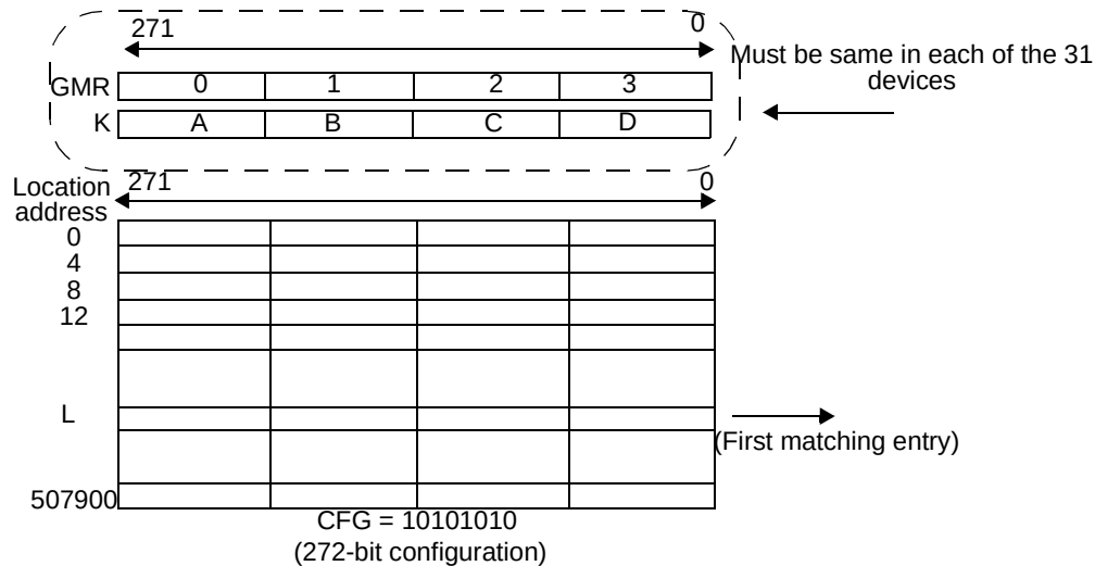
Figure 13-66. \times 272 Table with 31 Devices
