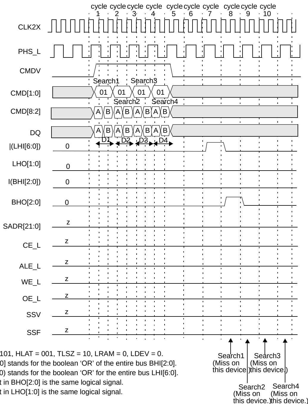
Figure 13-36. Timing Diagram for Devices Below the Winning Device in Block Number 1
