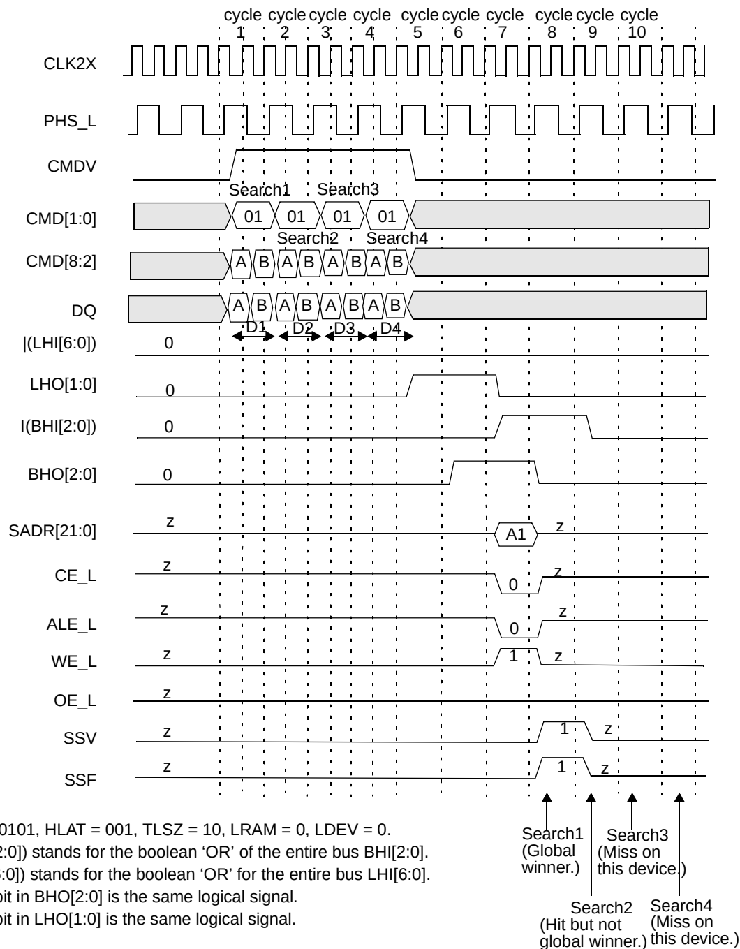
Figure 13-41. Timing Diagram for Globally Winning Device in Block Number 3
