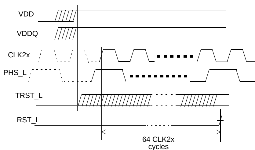
Figure 16-1. Power-up Sequence
