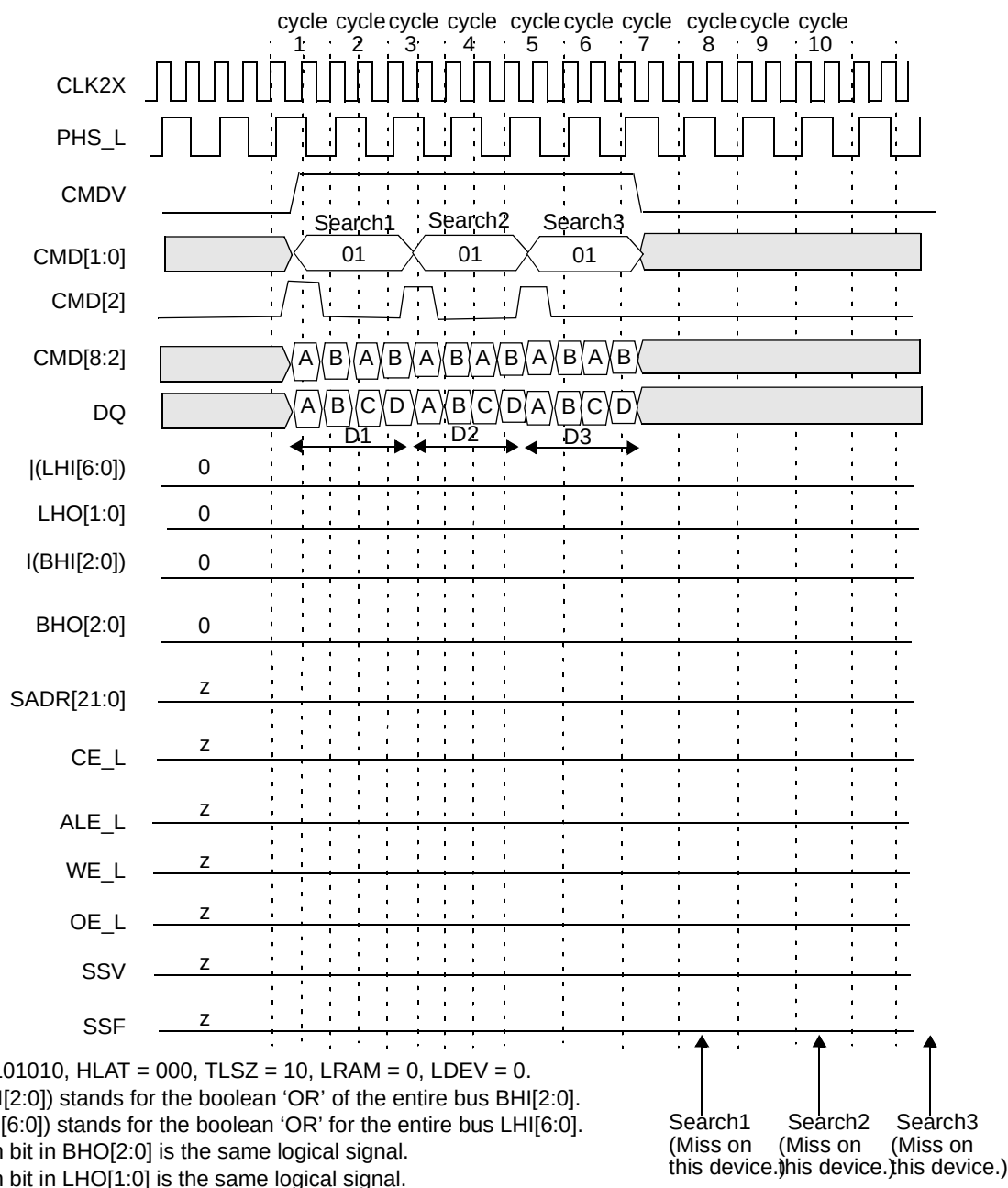
Figure 13-55. Timing Diagram for Each Device in Block Number 0 (Miss on Each Device)
