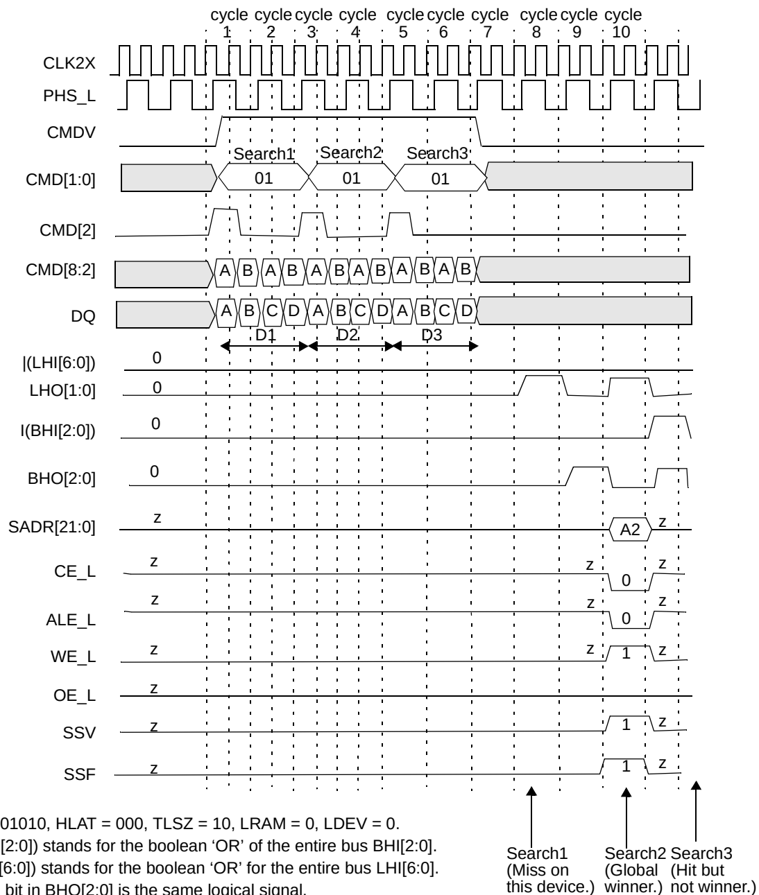
Figure 13-60. Timing Diagram for Globally Winning Device in Block Number 2
