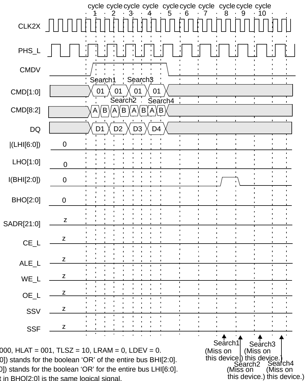
Figure 13-15. Timing Diagram for Devices Above the Winning Device in Block Number 2
