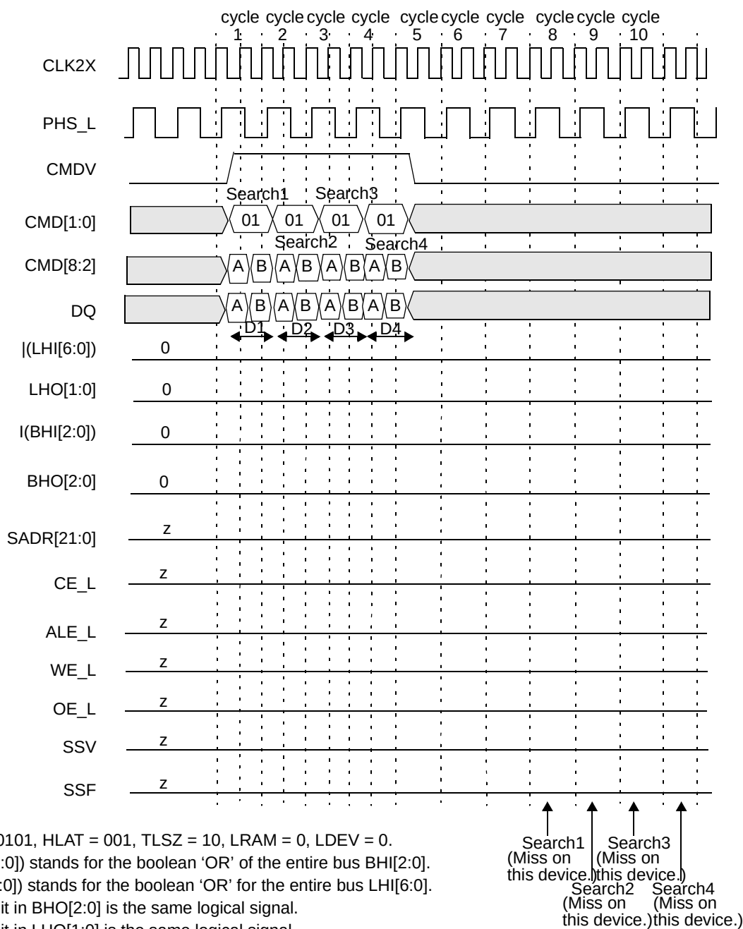
Figure 13-34. Timing Diagram for Each Device Above the Winning Device in Block Number 1
