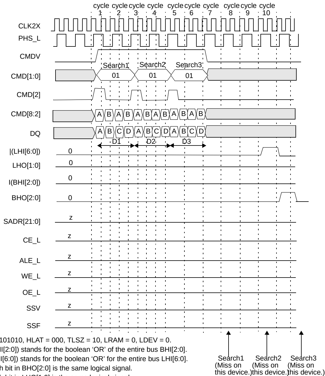
Figure 13-58. Timing Diagram for Devices Below the Winning Device in Block Number 1
