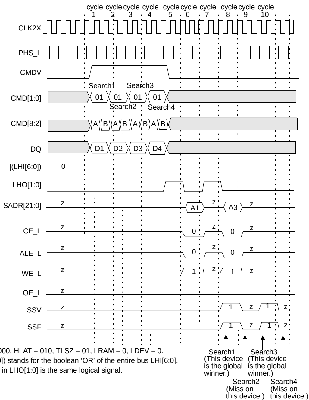
Figure 13-5. Timing Diagram for 68-bit Search Device Number 0
