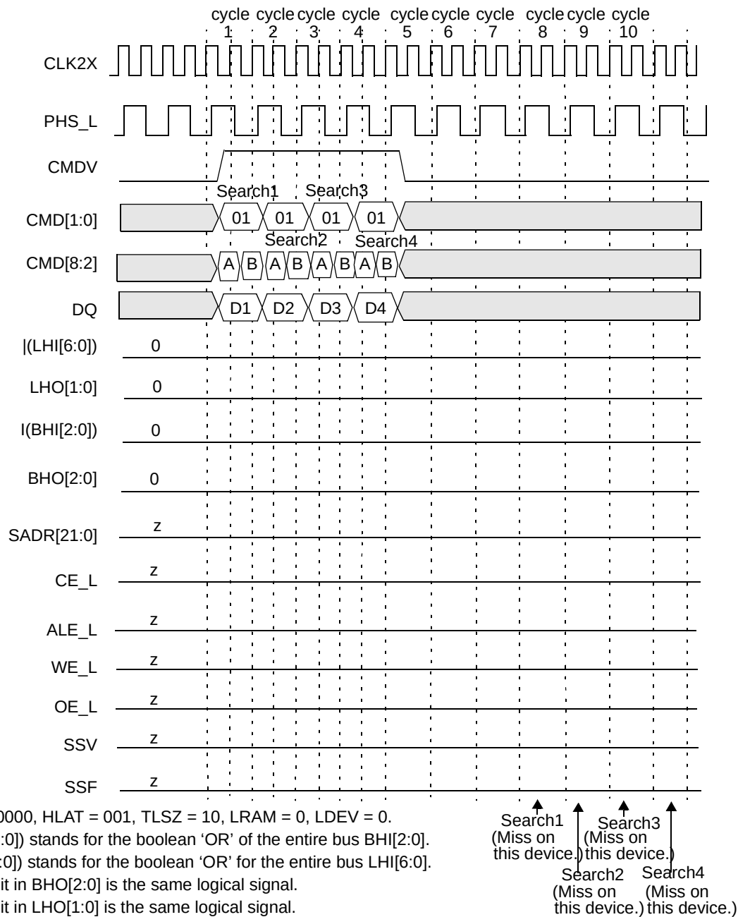
Figure 13-11. Timing Diagram for Each Device in Block Number 0 (Miss on Each Device)
