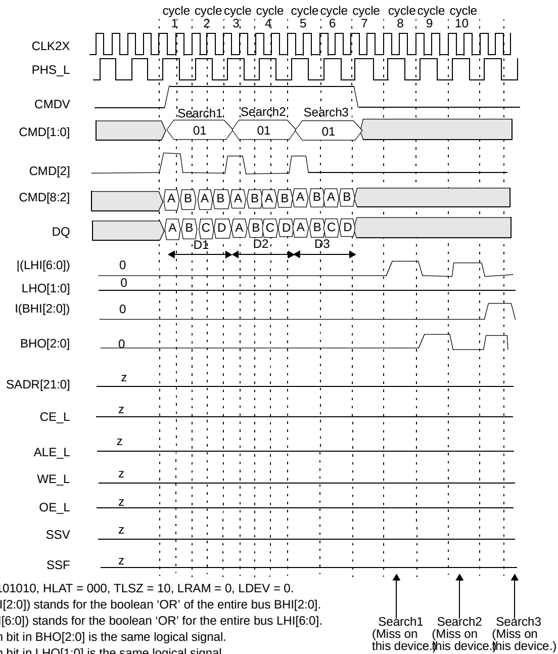
Figure 13-61. Timing Diagram for Devices Below the Winning Device in Block Number 2
