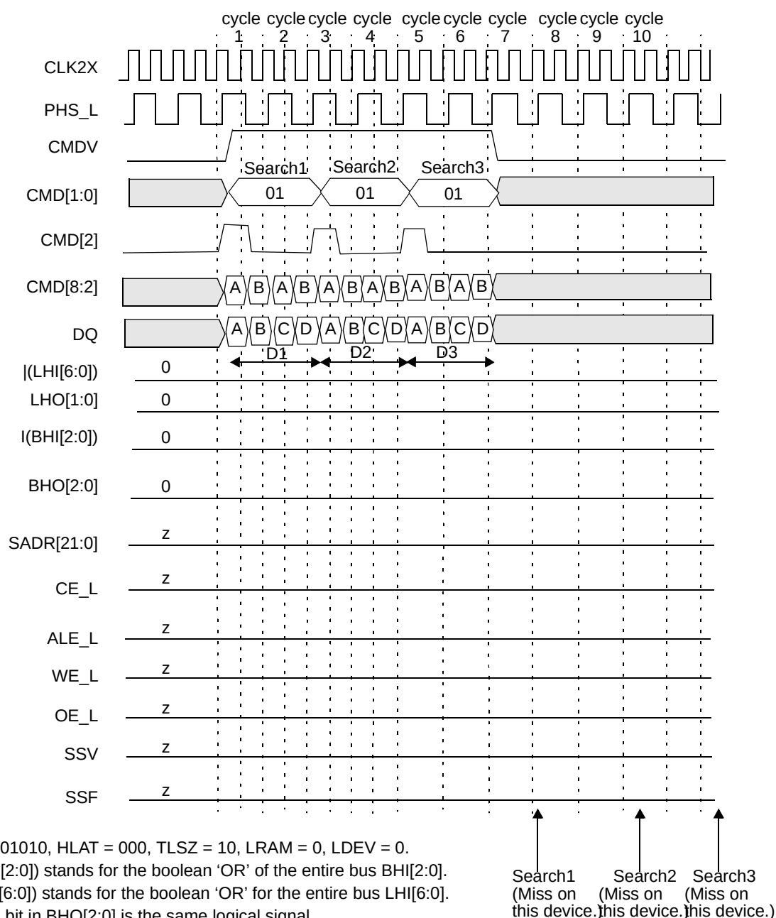
Figure 13-56. Timing Diagram for Each Device Above the Winning Device in Block Number 1
