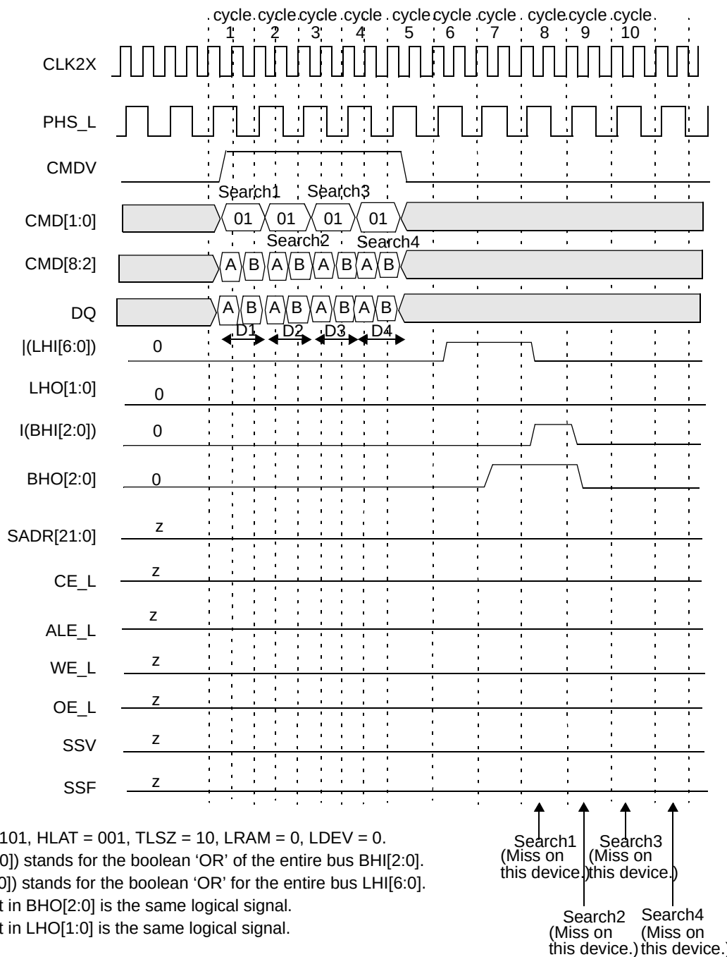
Figure 13-39. Timing Diagram for Devices Below the Winning Device in Block Number 2
