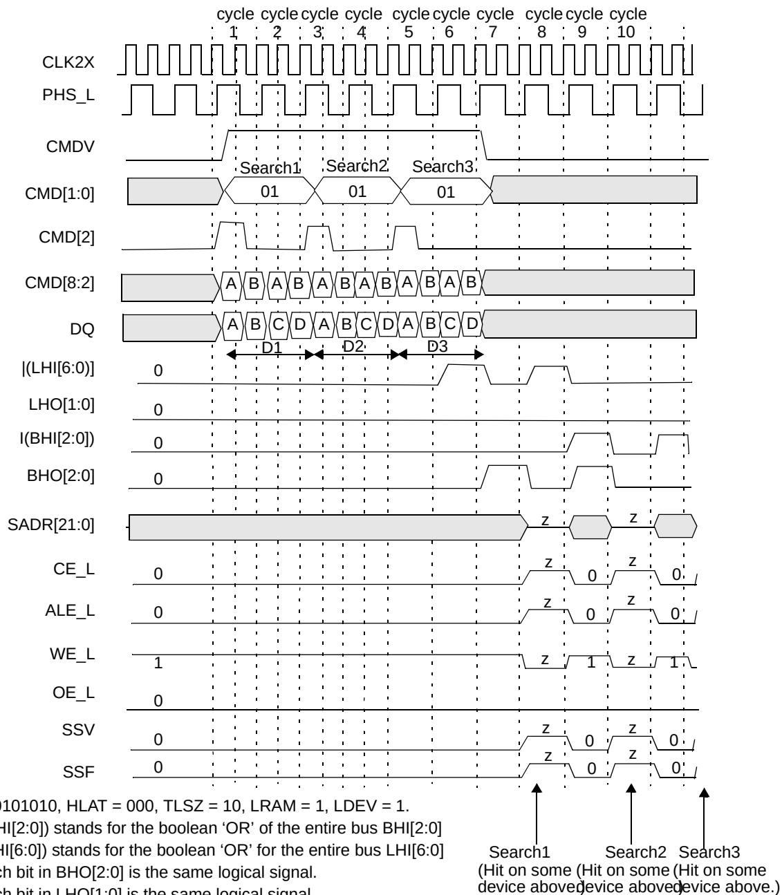
Figure 13-65. Timing Diagram of the Last Device in Block Number 3 (Device 30 in the Table)
