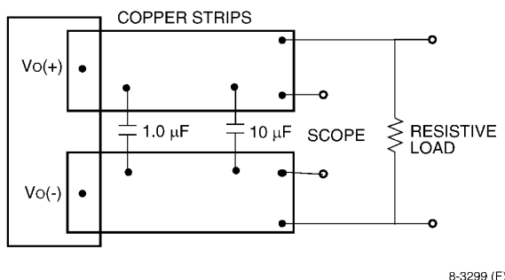
Figure 10. Input Reflected Ripple Current Test Setup.
