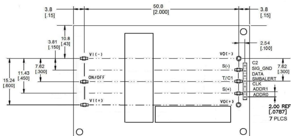
BOTTOM VIEW
