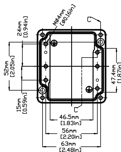
INTERIOR VIEW WITHOUT LID
