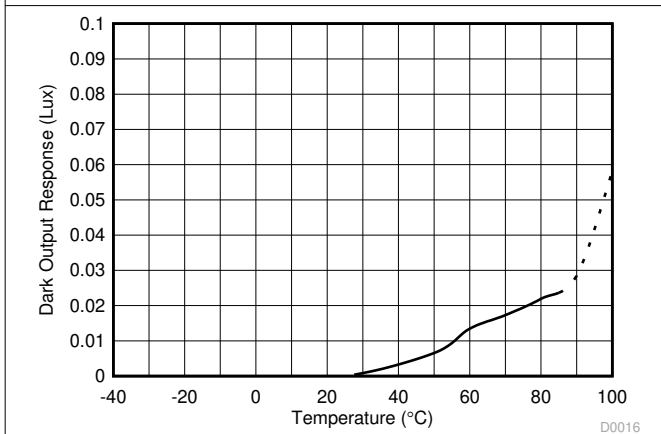
Figure 7-10. Dark Response vs Temperature
