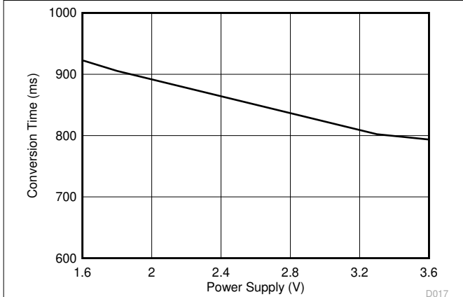
Figure 7-12. Conversion Time vs Power Supply
