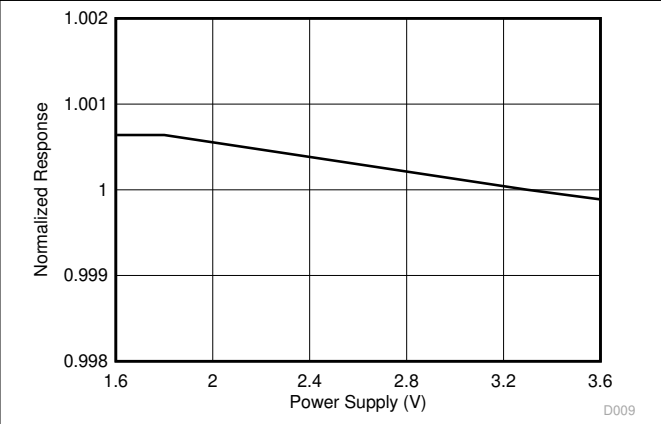
Figure 7-13. Normalized Response vs Power-Supply Voltage
