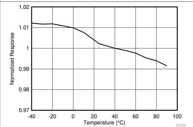
Figure 7-11. Normalized Response vs Temperature
