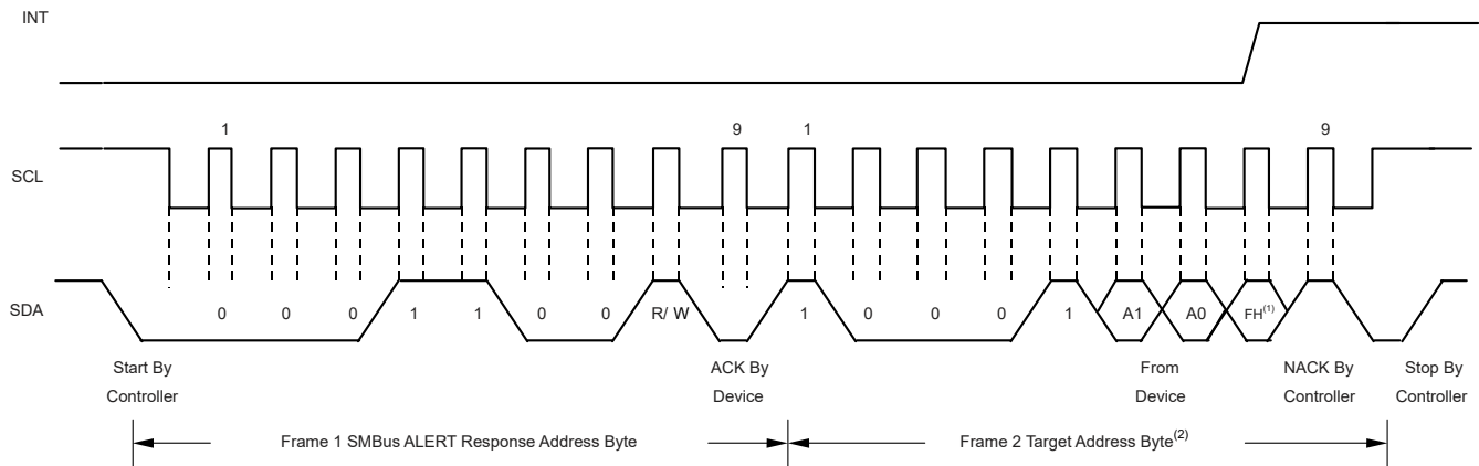
Figure 8-4. Timing Diagram for SMBus Alert Response
