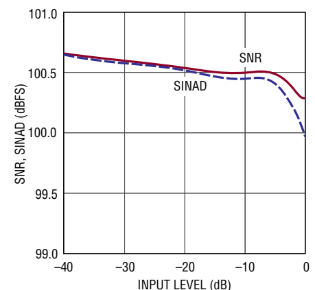
SNR, SINAD vs Input Level, f_{IN} = 1\text{kHz}
