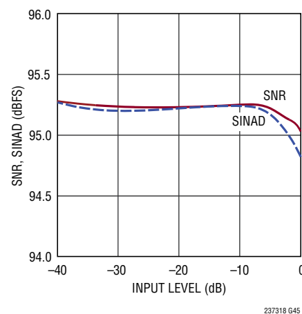
SNR, SINAD vs Input Level, f_{IN} = 1\text{kHz}
