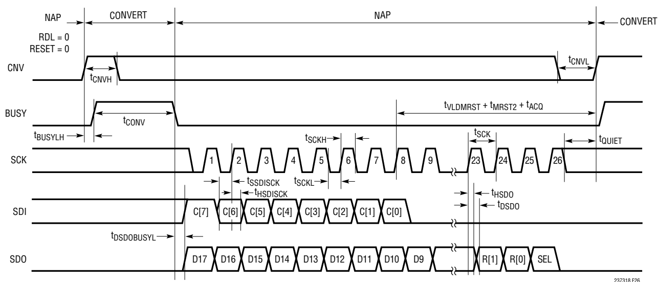
Figure 26. Using a Single LTC2373-18 Programming the Sequencer
