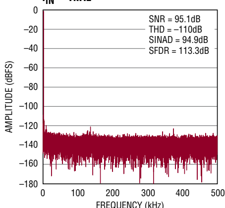
32k Point FFT f_{\text{SAMPL}} = 1\text{Mpsps} , f_{\text{IN}} = 1\text{kHz}
