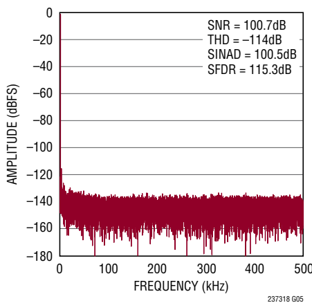
32k Point FFT f_{SAMPL} = 1\text{Mps} , f_{IN} = 1\text{kHz}
