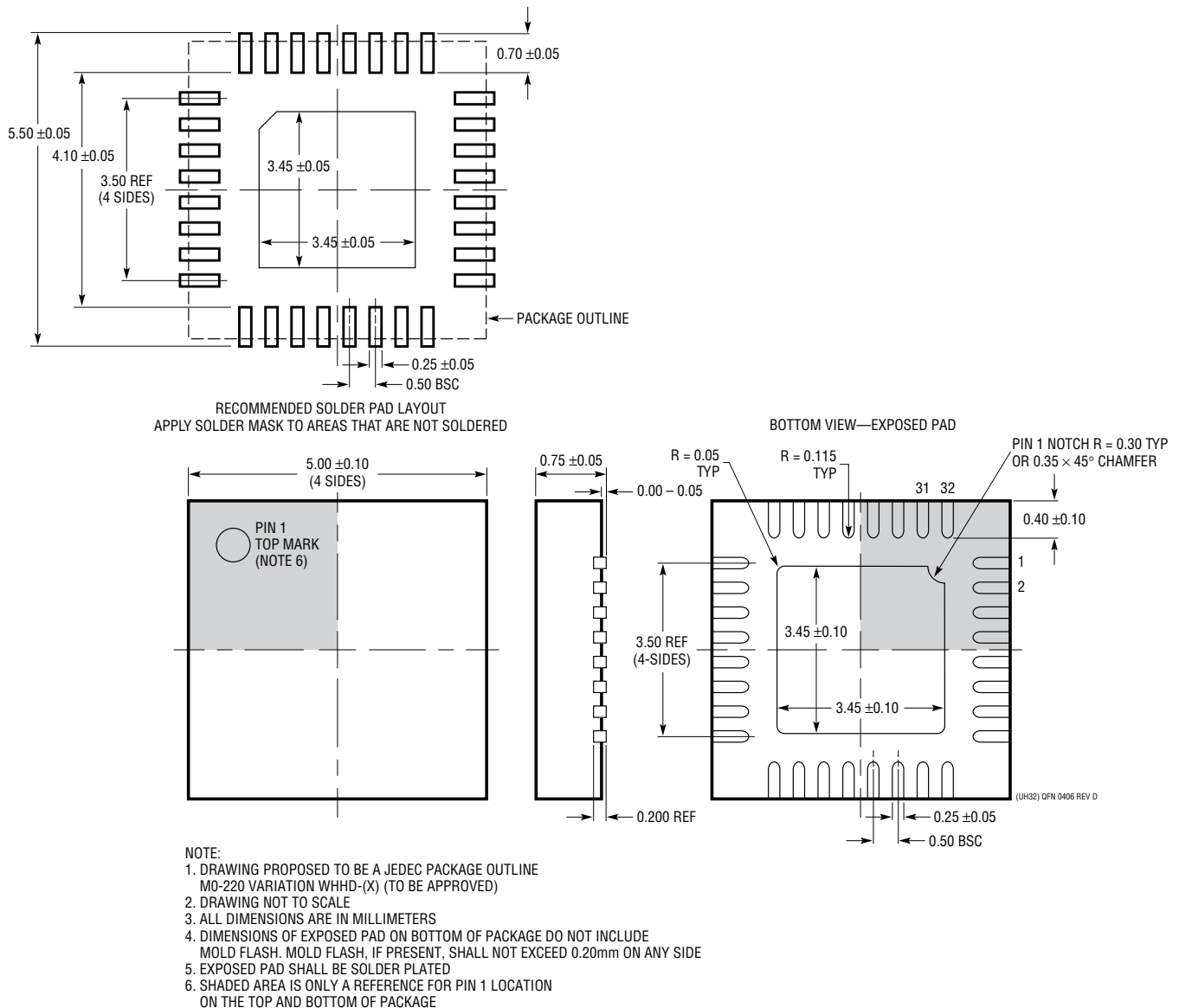
UH Package 32-Lead Plastic QFN (5mm × 5mm) (Reference LTC DWG # 05-08-1693 Rev D)
