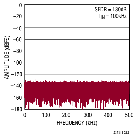
Crosstalk FFT (AC Crosstalk-Channel NOT Adjacent to MUXOUT)
