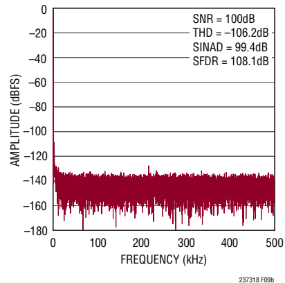
Figure 9b. 32k Point FFT f_{\text{SAMPL}} = 1\text{Mps} , f_{\text{IN}} = 1\text{kHz} for Circuit Shown in Figure 9a
