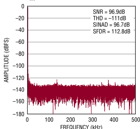
32k Point FFT f_{\text{SAMPL}} = 1\text{Mpsps} , f_{\text{IN}} = 1\text{kHz} , REFBUF = 5\text{V}
