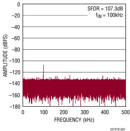
Crosstalk FFT (AC Crosstalk-Channel Adjacent to MUXOUT)
