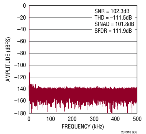
32k Point FFT f_{SAMPL} = 1\text{Mps} , f_{IN} = 1\text{kHz} , REF_{BUF} = 5\text{V}
