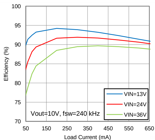
Figure 3. Efficiency at 200kHz, 10V
