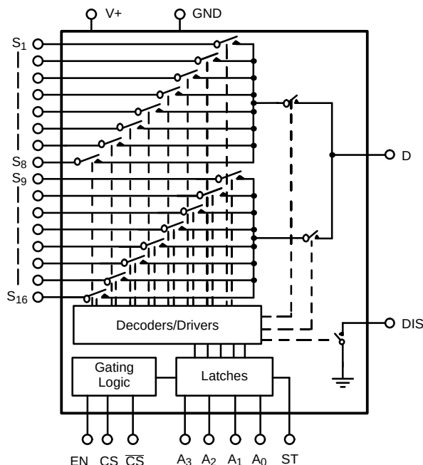
FIGURE 1. DG535/536 Functional Block Diagram
