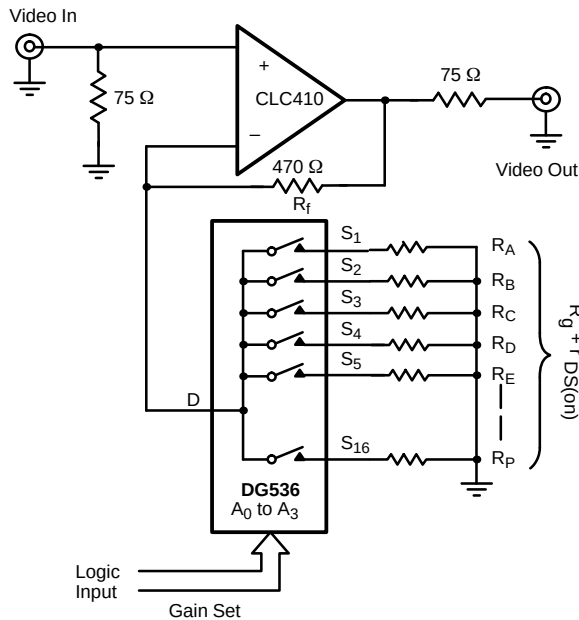
FIGURE 19. Programmable Gain Video Amplifier
