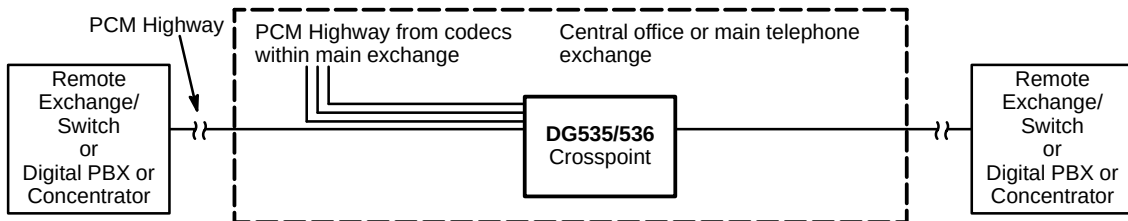
FIGURE 17. DG536 PCM Distribution Frame
