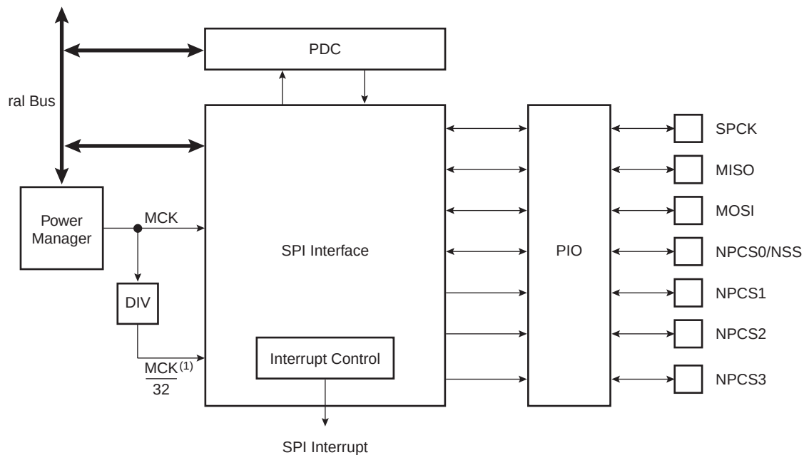
Figure 23-1. Block Diagram
