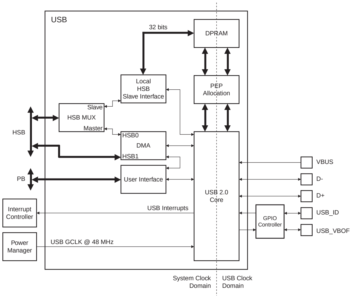
Figure 30-1. Block Diagram
