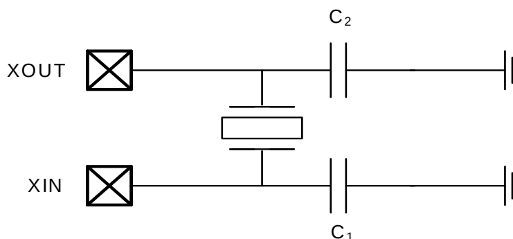
Figure 13-2. Oscillator connections
