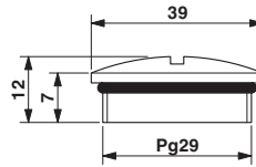
Dimensioned drawing
