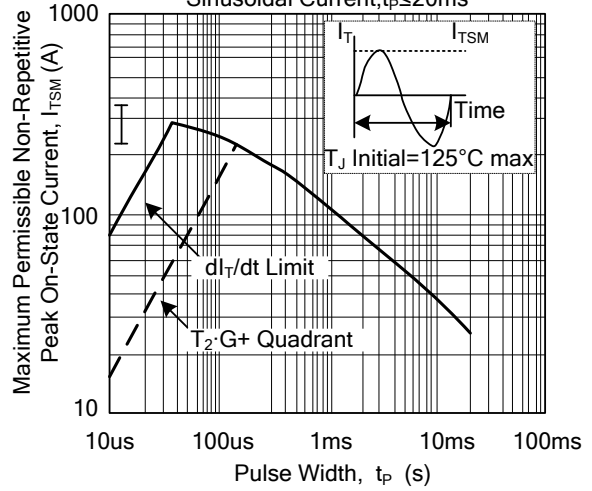
Maximum Permissible Non-Repetitive On-State Current, I_{TSM} , vs Pulse Width t_p , for Sinusoidal Current, t_p \leq 20ms
