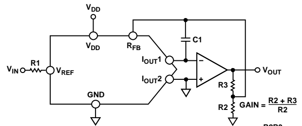
Figure 42. Increasing Gain of Current Output DAC
