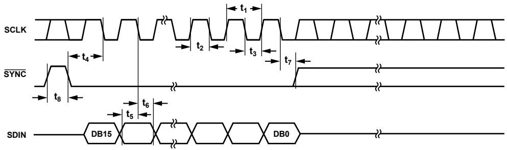
Figure 2. Standalone Timing Diagram
