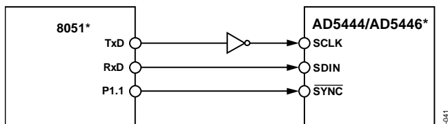
Figure 50. 80C51/80L51 to AD5444/AD5446 Interface
