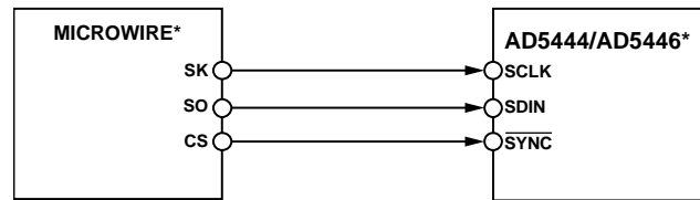
Figure 52. MICROWIRE to AD5444/AD5446 Interface
