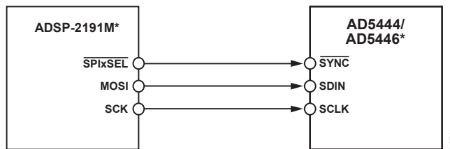
Figure 46. ADSP-2191M SPI to AD5444/AD5446 Interface
