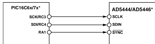
Figure 53. PIC16C6x/7x to AD5444/AD5446 Interface
